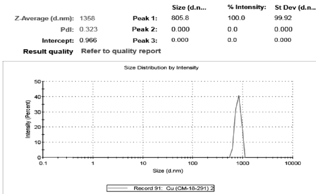
Fig. 2. Size distribution intensity of synthesized Cu-NPs.
