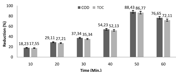
Fig. 10. Effect of reaction contact time on water quality parameters.
