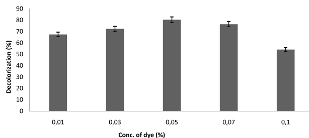
Fig. 4. Effect of concentration of Reactive Blue 19 dye on its decolorization (%) using copper nanoparticles.
