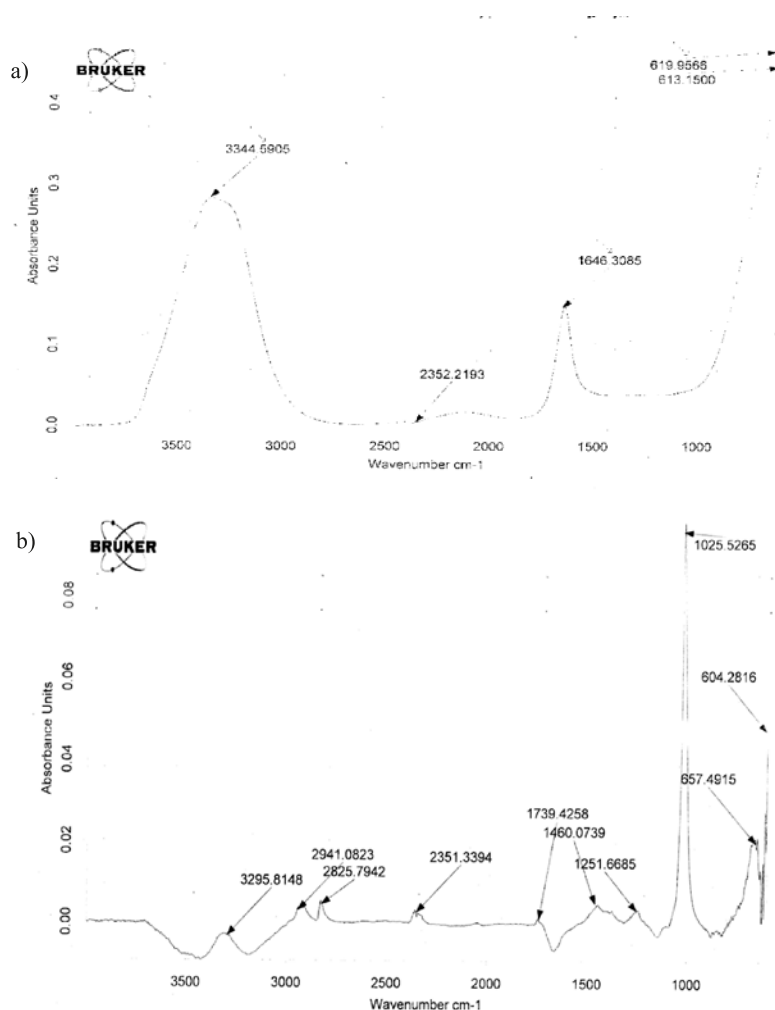
Fig. 9. a) FTIR spectrum of reactive dye 222 before catalytic treatment, b) FTIR spectrum of reactive dye 222 after catalytic treatment.
