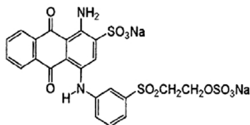
Structure of Reactive Blue 19 dye
