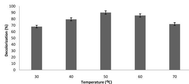
Fig. 7. Effect of temperature on decolorization (%) of Reactive Blue 19 dye using copper nanoparticles.
