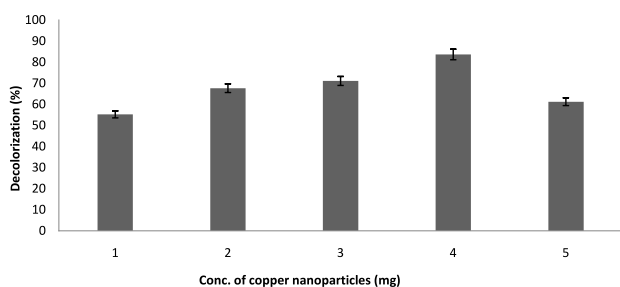
Fig. 5. Effect of concentration of copper nanoparticles on decolorization (%) of Reactive Blue 19 dye.
