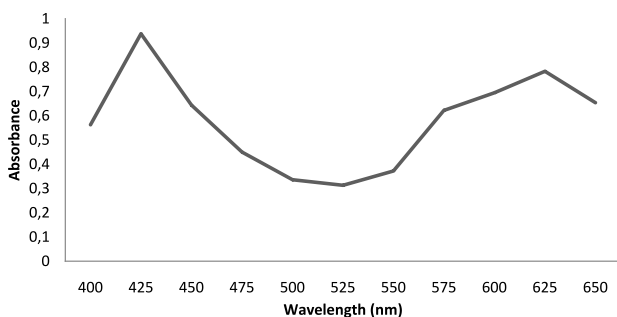
Fig. 3. Determining wavelength of maximum absorbance for Reactive Blue 19 dye.
