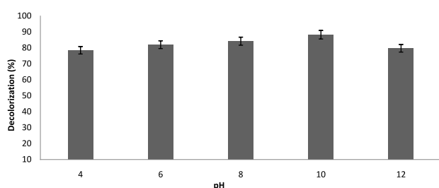
Fig. 6. Effect of pH on decolorization (%) of Reactive Blue 19 dye using copper nanoparticles.
