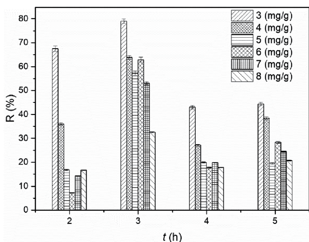
Fig. 4. Effect of reaction time and initial concentration on Cr(VI) adsorption by PGA-PL-tannin gel.
