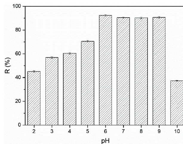
Fig. 3. Effect of initial pH on Cr(VI) adsorption by PGA-PL-tannin gel.
