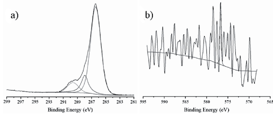
Fig. 6. XPS spectra of Cr(VI) adsorbed gel: a) gel C1s; b) gel after adsorption of Cr(VI).
