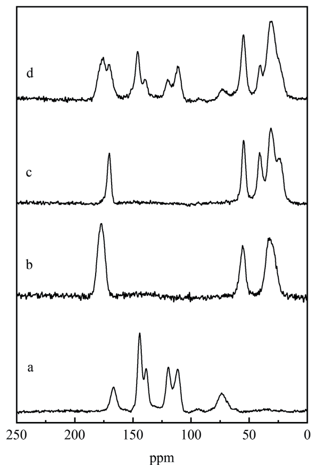
Fig. 2. Solid-state ^{13}\text{C} -NMR spectrum of the gel: a) tannic acid; b) \epsilon -PL; c) \gamma -PGA; d) PGA-PL-tannin gel.
