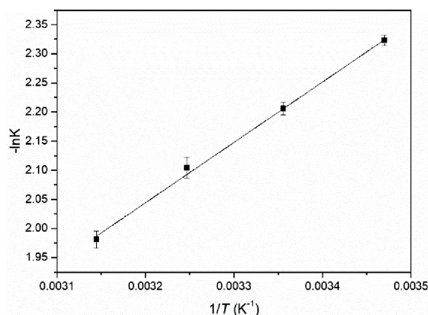
Fig. 5. Plots of -\ln K vs. 1/T for the adsorption of Cr(VI) by PGA-PL-tannin gel.
