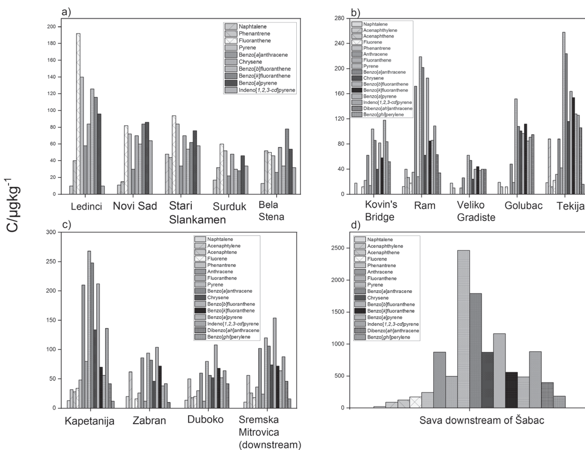
Fig. 2. PAHs in: a) Danube River sediments - part 1, b) Danube River sediments - part 2, c) Sava River sediments, and d) Sava River sediments downstream of Šabac.
