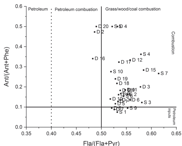
Fig. 4. Diagnostic ratio plots of Fla/(Fla+Pyr) vs. Ant/(Ant+Phe) in Danube and Sava river sediments.
