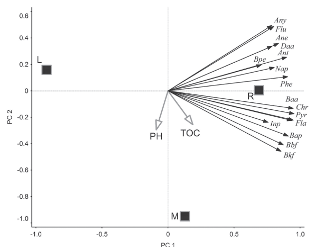
Fig. 3. Principal component analysis showing the relationship between PAHs, side of the river (squares: R-right, L-left, M-middle), TOC and pH (PC1).
