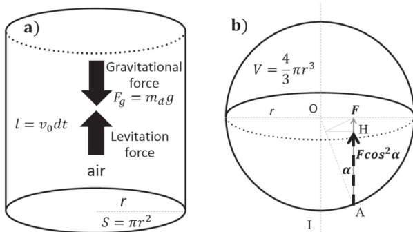
Fig. 1. Forces exerted on a microparticle that is assumed to be a sphere.
