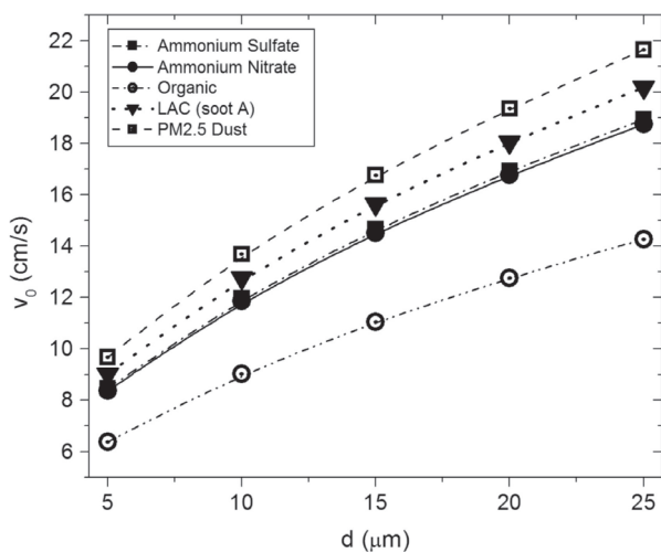
Fig. 2. Minimum speed of air v_0 from Eq. (6) to levitate the dust for five samples.
