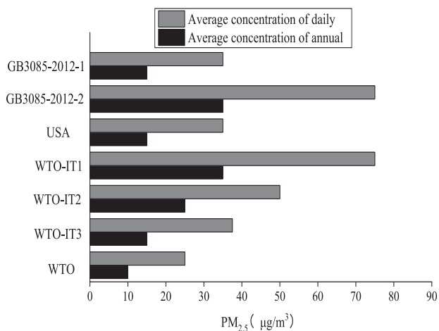
Fig. 1. Rules for PM_{2.5} concentration by different air quality standards.
