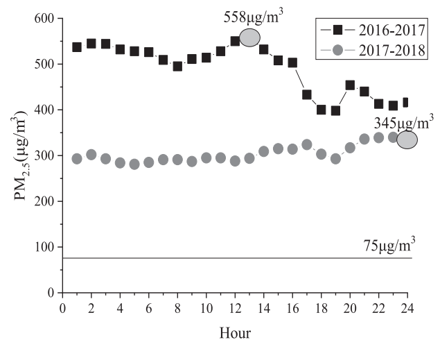
Fig. 3. Daily characteristics of PM_{2.5} pollution.
