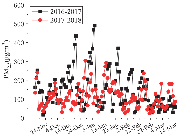
Fig. 2. Monthly characteristics of PM_{2.5} pollution.
