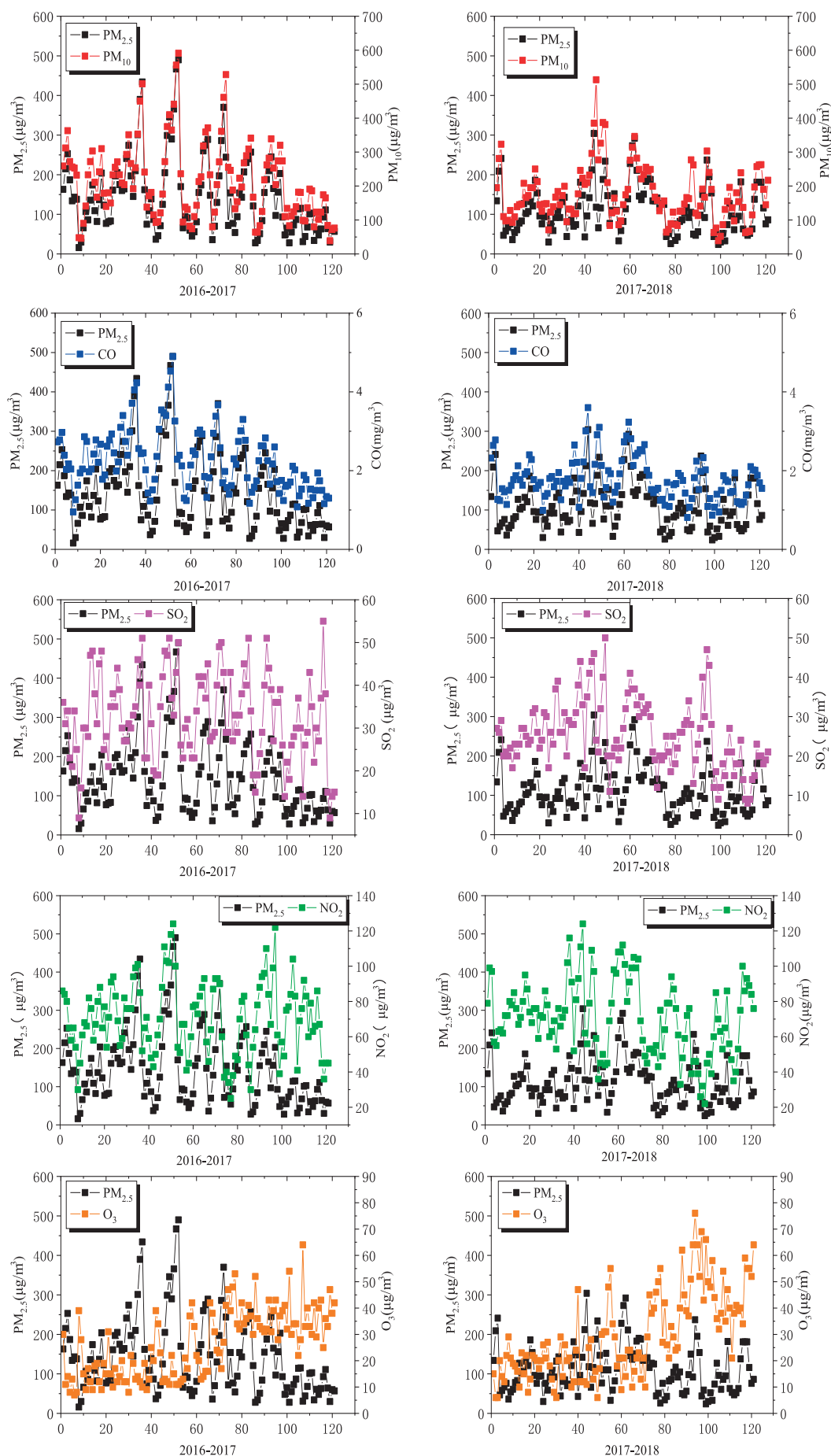
Fig. 5. Correlativity between PM_{2.5} and other pollutants.
