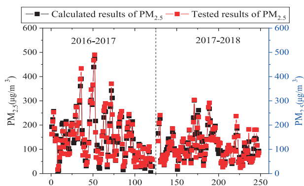
Fig. 6. Comparison of calculated and tested results of PM_{2.5} .
