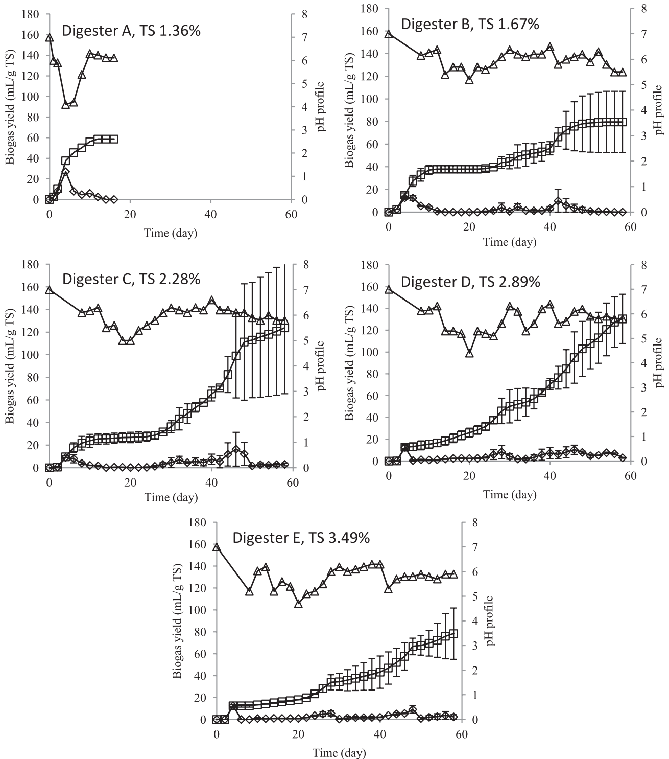
Fig. 1. The effect of total solid concentration on biogas production daily ( \diamond ), biogas production cumulative ( \square ), pH profile ( \Delta ).
