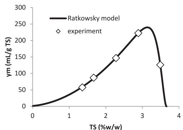
Fig. 4. Correlation between TS level on biogas yield based on Ratkowsky Model.
