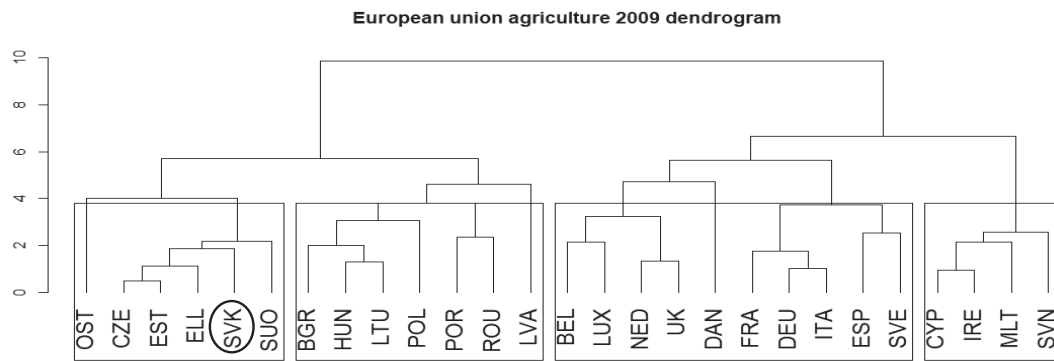
Fig. 1. Dendrogram of EU Member States based on 2009 environmental indicators.
