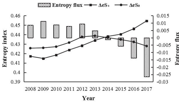
Fig. 3. Entropy flux of RPSS in China from 2008 to 2017.
