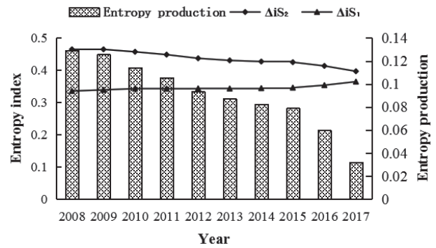
Fig. 4. Entropy production of RPSS in China from 2008 to 2017.
