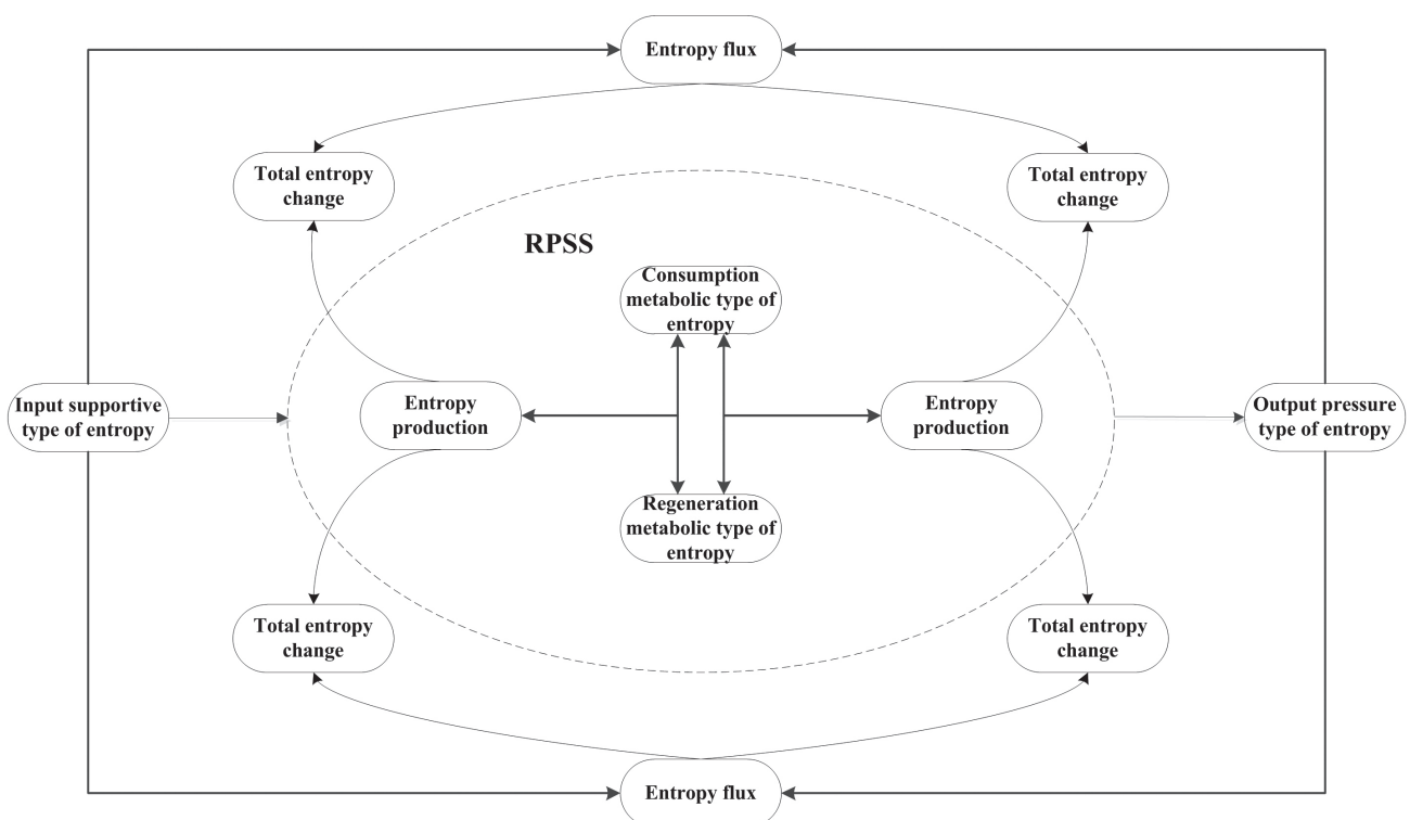
Fig. 2. Entropy change mode of RPSS [22]. (The figure is derived from the research results of our team and has been modified).
