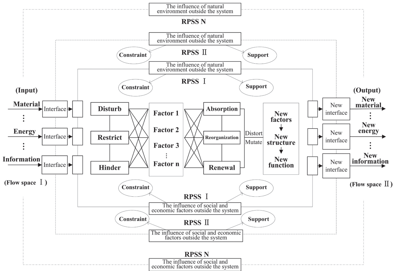
Fig. 1. Flow-driven model for the evolution of RPSS [28]. (The figure is derived from the research results of our team and has been modified).
