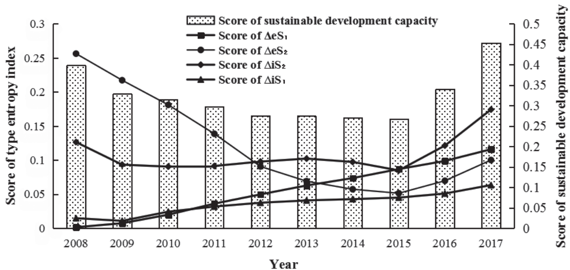
Fig. 5. Score of sustainable development capacity of RPSS in China from 2008 to 2017.
