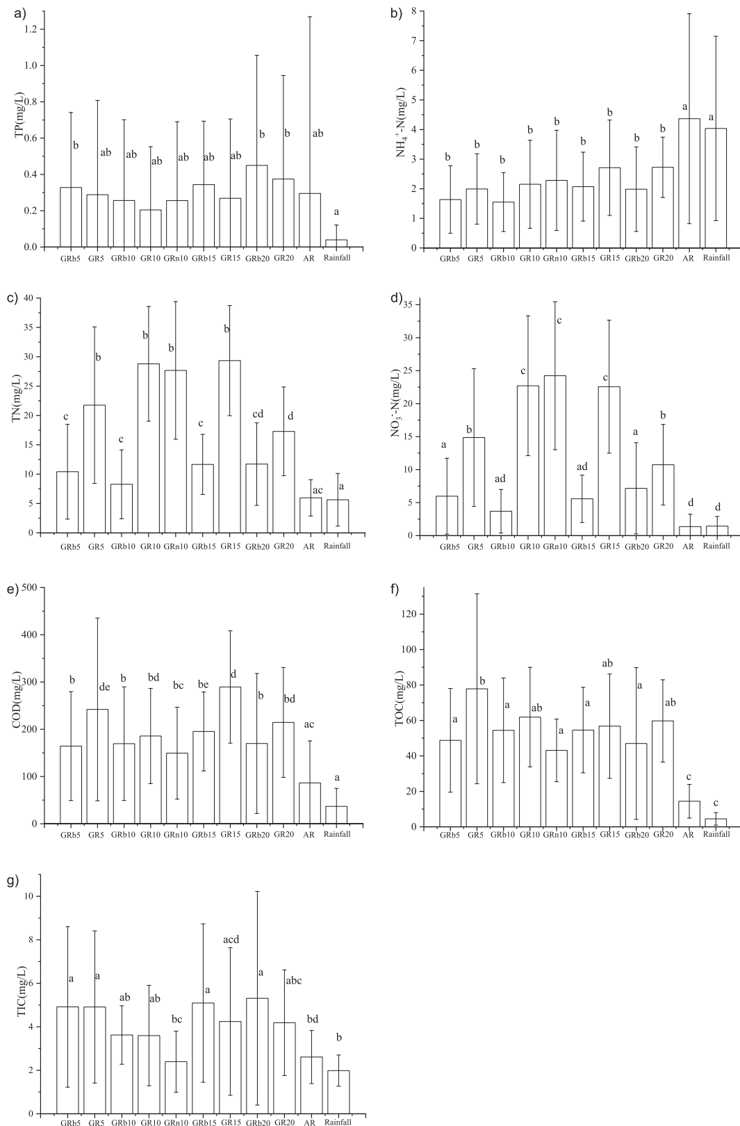
Fig. 4. The average TP, NH 4 + -N, NO 3 - -N, TN, COD, TOC and TIC concentrations of monitoring rainfall events from the green roof, asphalt roof, and rainfall.
