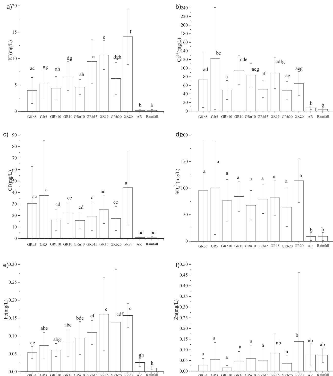
Fig. 5. The average K + , Ca 2+ , Cl - , SO 4 2- , Fe and Zn concentrations of monitoring rainfall events from the green roof, asphalt roof, and rainfall.
