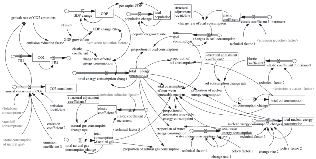
Fig. 2. System Flow Diagram of Energy Consumption Structure Prediction Model.
