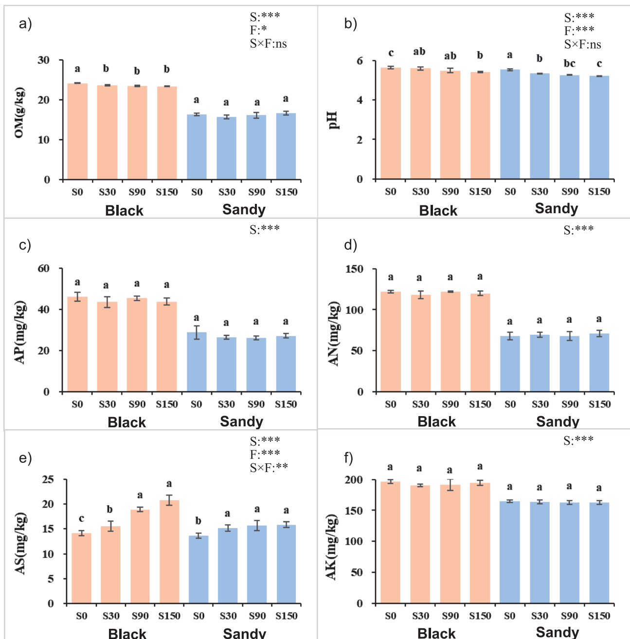
Fig. 1. The physicochemical properties of the soil vary with the amount of S fertilizer applied. In order to measure the overall impact of soil type (S), fertilizers (F) and their interaction (S×F) on soil variables, two-way ANOVAs was carried out. Different lowercase letters indicate significant differences between treatments estimated by one-way ANOVA and Duncan's multiple-range test and asterisks denote significant differences at p < 0.05 , p < 0.01 and p < 0.001 probability levels (*, ** and ***).
