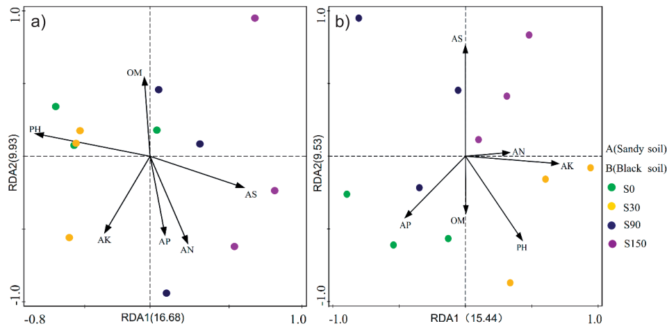
Fig. 5. Redundancy analysis (RDA) revealed the influence of soil properties on the structure of soil bacterial community, A(Sandy soil), B(Black soil). The green, yellow, blue, and purple circles represent different S application rates (S0, S30, S90, S150), Soil properties OM represent soil organic matter and AS represents available sulfur.
