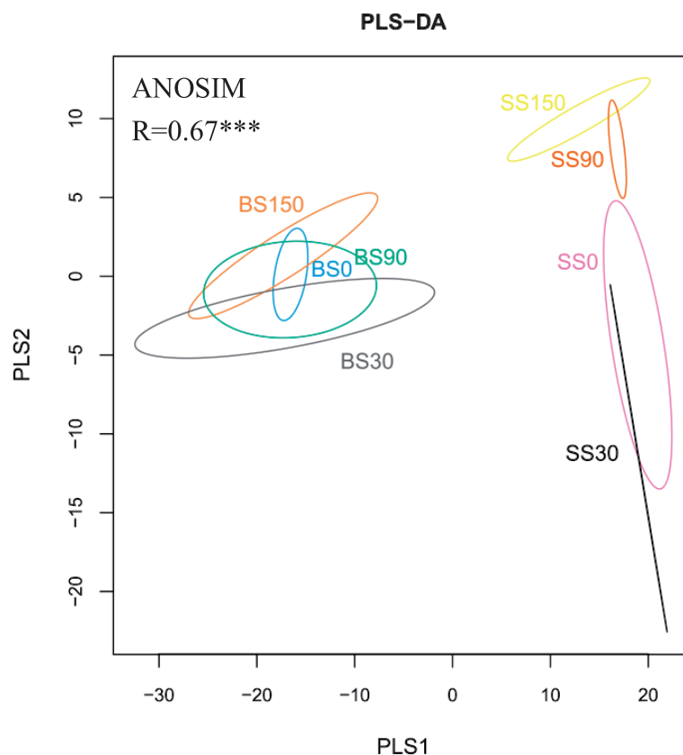
Fig. 4. Partial Least Squares Discriminant Analysis (PLS-DA) of different soil types and S fertilizer rates on soil bacterial communities.
