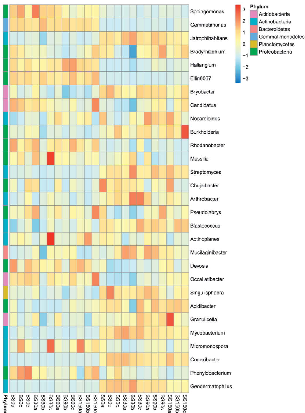
Fig. 3. The heatmap shows the bacterial taxonomic variations (genus level with abundance greater than 0.1%) over S fertilization and soil types., the asterisk (*) indicates the p < 0.05 , p < 0.01 and p < 0.001 (*, ** and ***) according to the Pearson correlation between their relative abundances and AS application rates.
