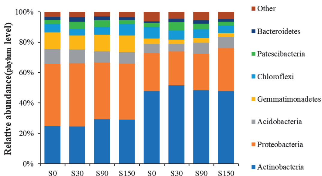
Fig. 2. The relative abundance levels of the dominant phylum under different treatments of the two soil types. In order to measure the overall impact of soil type (S), fertilizers (F) and their interaction (S×F) on phylum level bacterial community composition, two-way ANOVAs was carried out. Asterisks denote significant differences at p < 0.05 , p < 0.01 and p < 0.001 probability levels (*, **and***).
