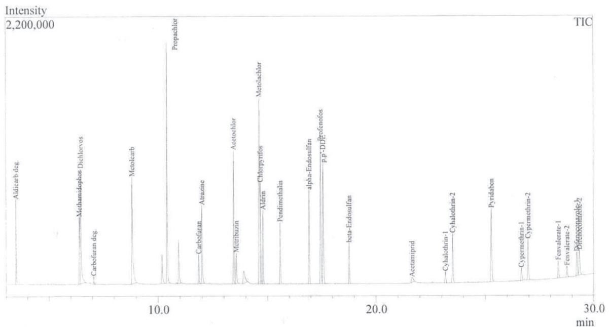
Fig. 4. GC-MS chromatogram of the Standard Pesticides.
