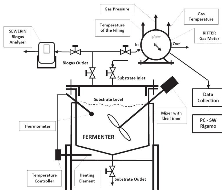
Fig. 1. Schematic representation of the technological process of the biogas production.
