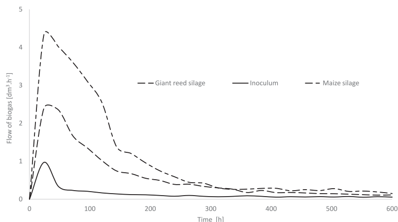
Fig. 2. Biogas flow production from individual types of input mixtures.
