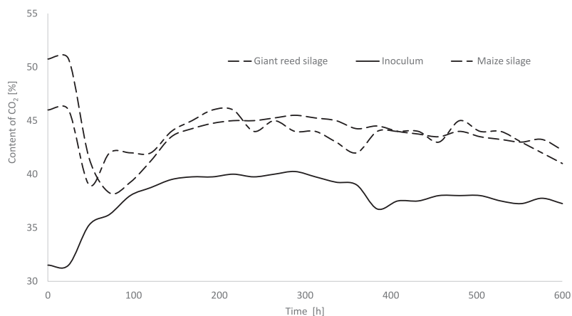
Fig. 4. Carbon dioxide content in the biogas of individual types of input mixtures.
