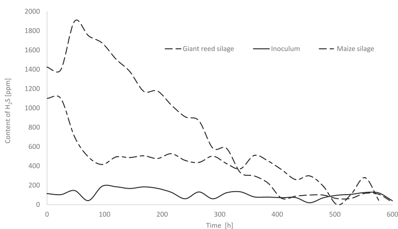
Fig. 5. Hydrogen sulphide content in the biogas of individual types of input mixtures.
