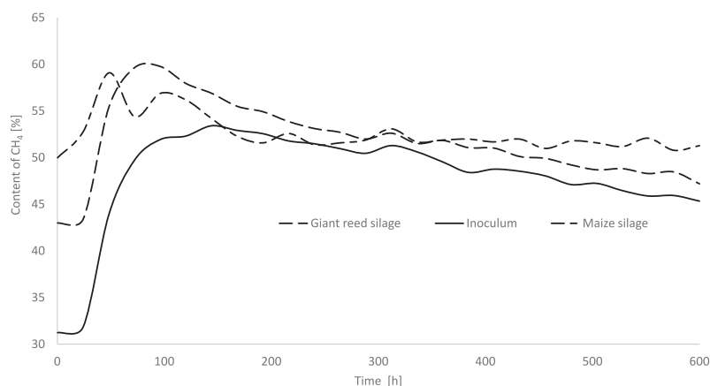
Fig. 3. Methane content in the biogas produced from individual types of input mixtures.
