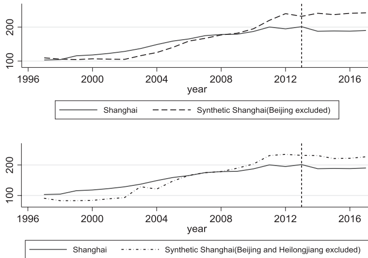
Fig. 5. Leave-one-out sensitivity analysis.
