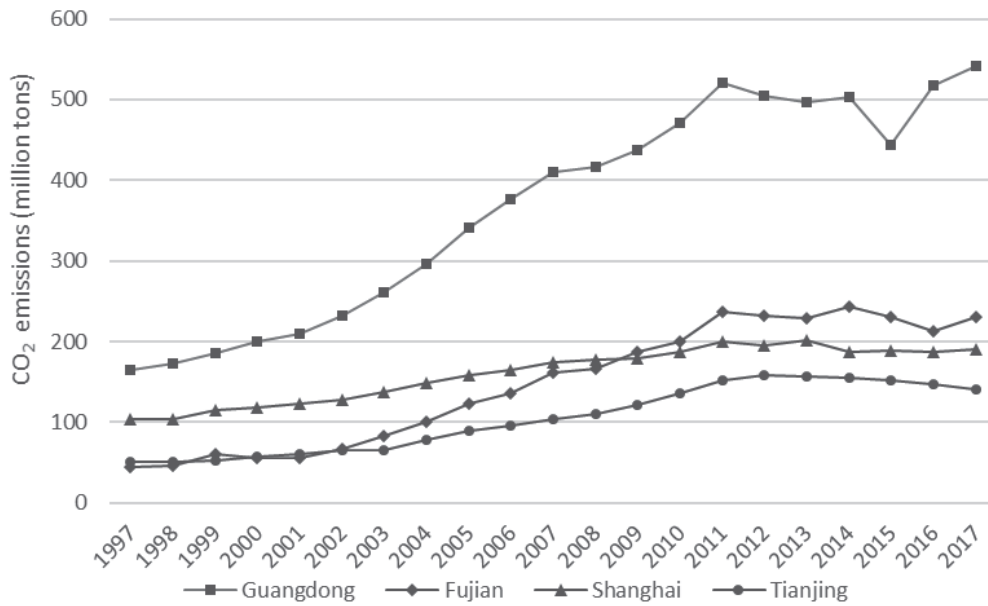
Fig. 1. CO 2 emissions in the Provinces and municipalities which established FTZs.
