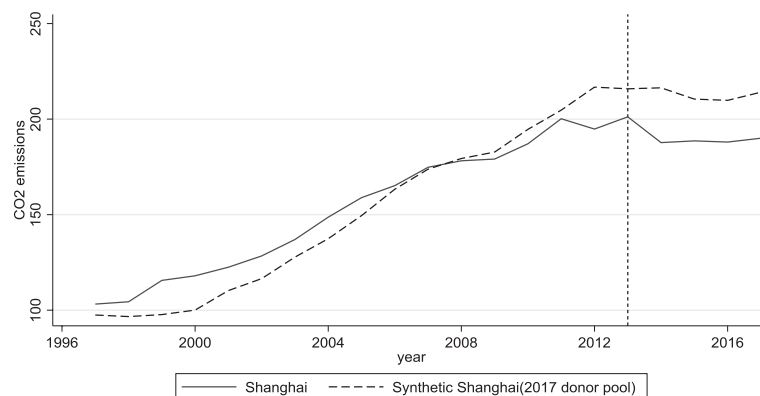
Fig. 3. Trends in CO 2 emissions: Shanghai vs. Synthetic Shanghai (2017 donor pool).
