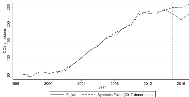
Fig. 7. Trends in CO 2 emissions: Fujian versus Synthetic Fujian.
