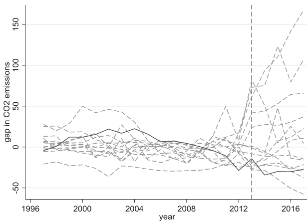
Fig. 4. CO 2 emissions gaps in Shanghai and placebo gaps in other control provinces or municipalities.
