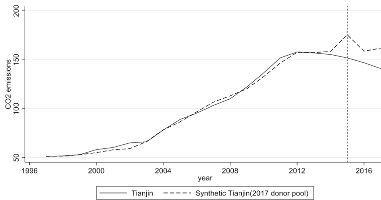
Fig. 6. Trends in CO 2 emissions: Tianjin versus Synthetic Tianjin.
