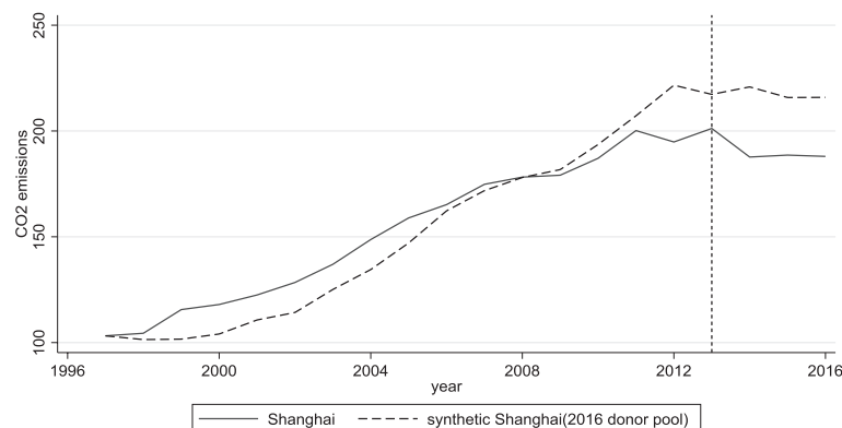
Fig. 2. Trends in CO 2 emissions: Shanghai vs. Synthetic Shanghai (2016 donor pool).
