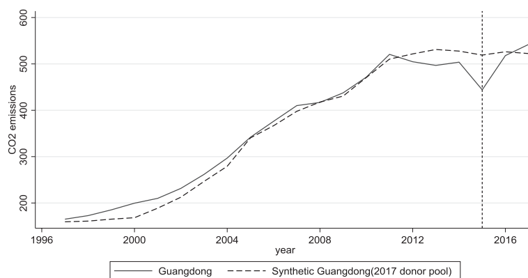
Fig. 8. Trends in CO 2 emissions: Guangdong versus Synthetic Guangdong.
