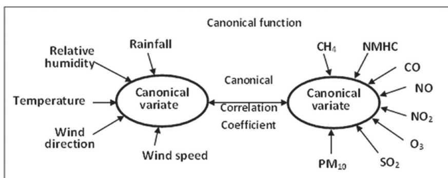
Fig. 2. The components of canonical function.
