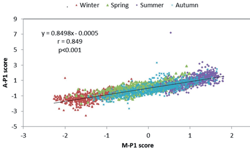
Fig. 3. Relationship between meteorological variate M-P1 and air pollutants variate A-P1 according to season.
