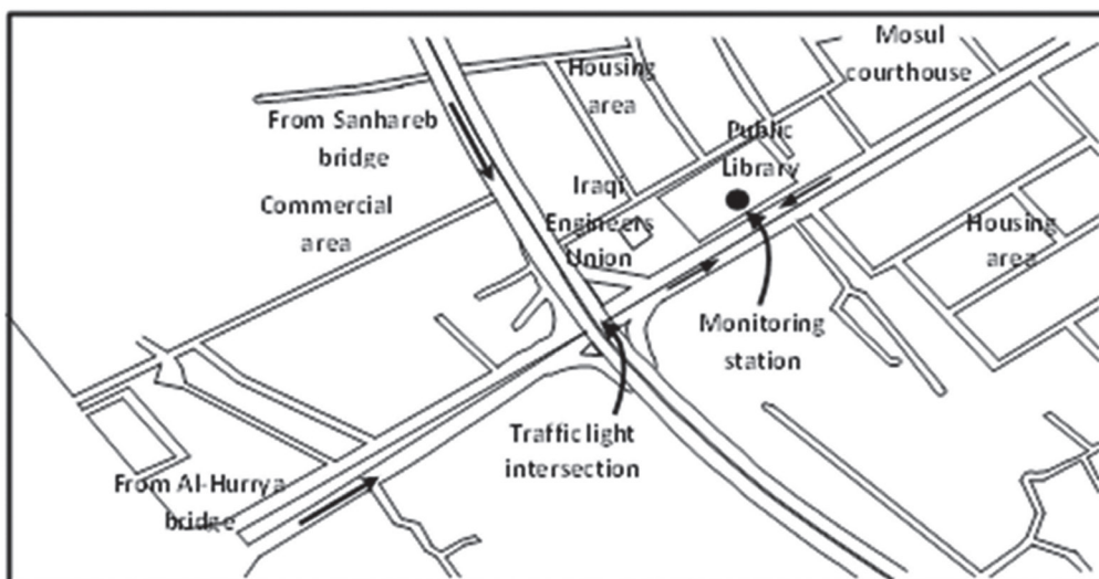
Fig. 1. Location of the study site with monitoring station.
