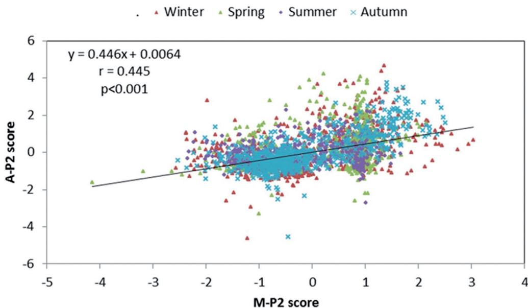
Fig. 4. Relationship between meteorological variate M-P2 and air pollutants variate A-P2 according to season
