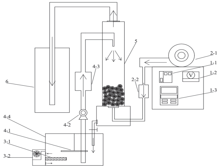
Fig. 1. Schematic diagram of ammonia nitrogen stripping device.
