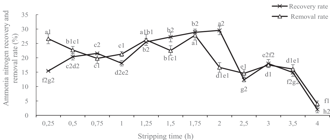
Fig. 2. Ammonia nitrogen recovery and removal rate in different time periods.
