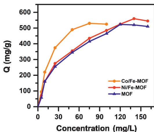
Fig. 5. Effect of initial concentration of CR colorant on the adsorption capacity of M/Fe-MOF materials (M=Co, Ni).
