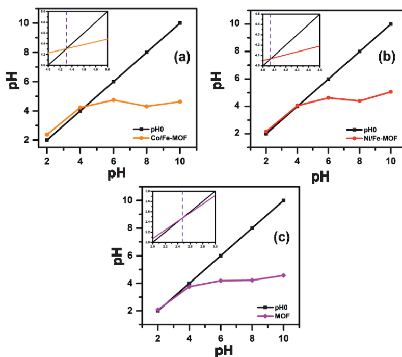
Fig. 1. Isoelectric curves of the materials a) Co/Fe-MOF, b) Ni/Fe-MOF, c) Fe-MOF.
