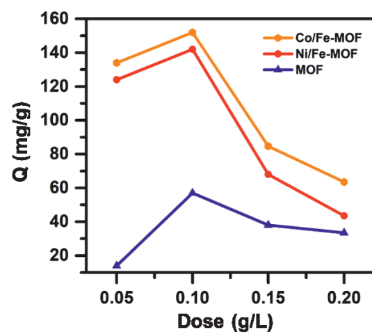
Fig. 4. Effect of amount of adsorbent on the adsorption capacity of M/Fe-MOF materials (M=Co, Ni).
