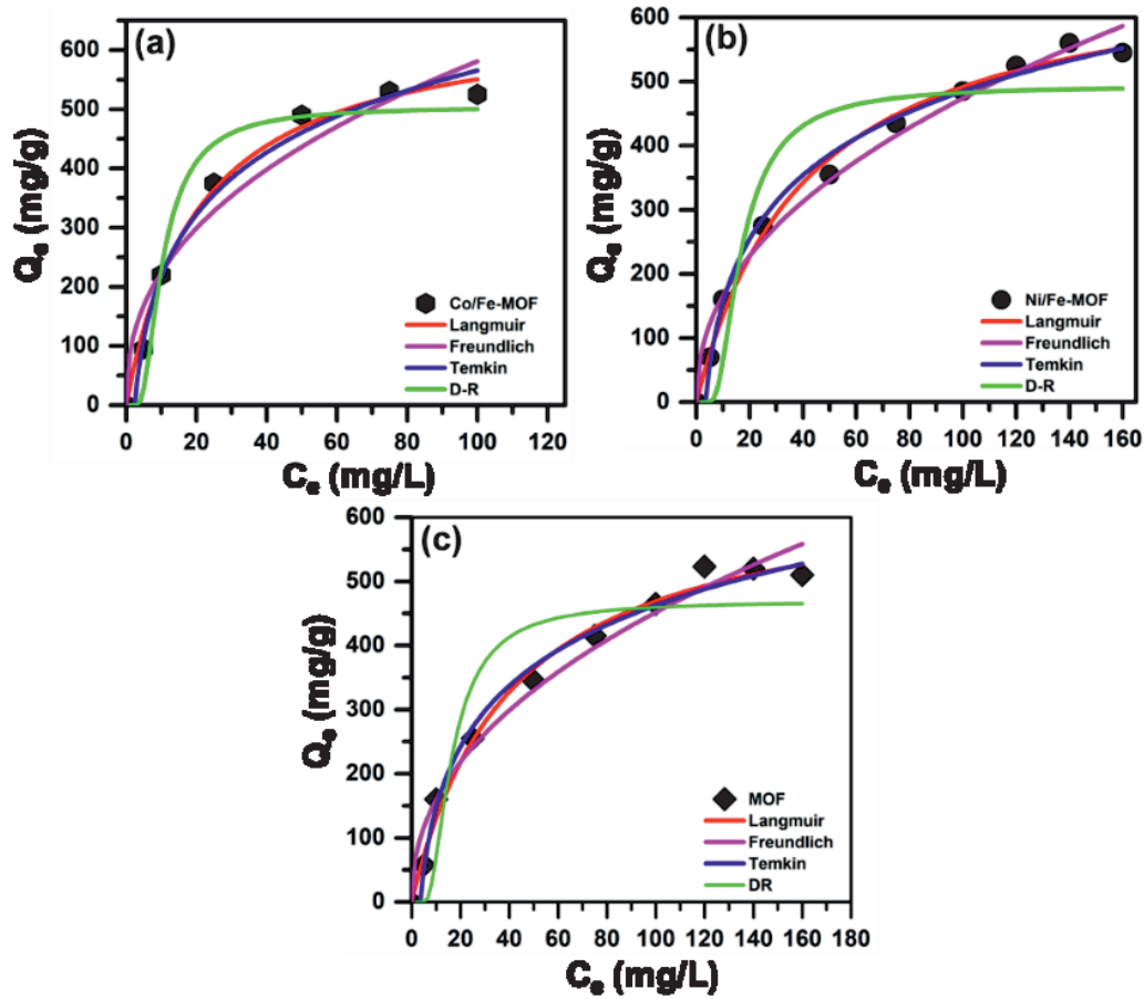
Fig. 6. The adsorption isotherm model of the materials a) Co/Fe-MOF, b) Ni/Fe-MOF, c) Fe-MOF.
