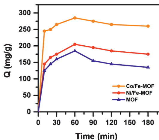
Fig. 3. Effect of time on the adsorption capacity of M/Fe-MOF materials (M=Co, Ni).
