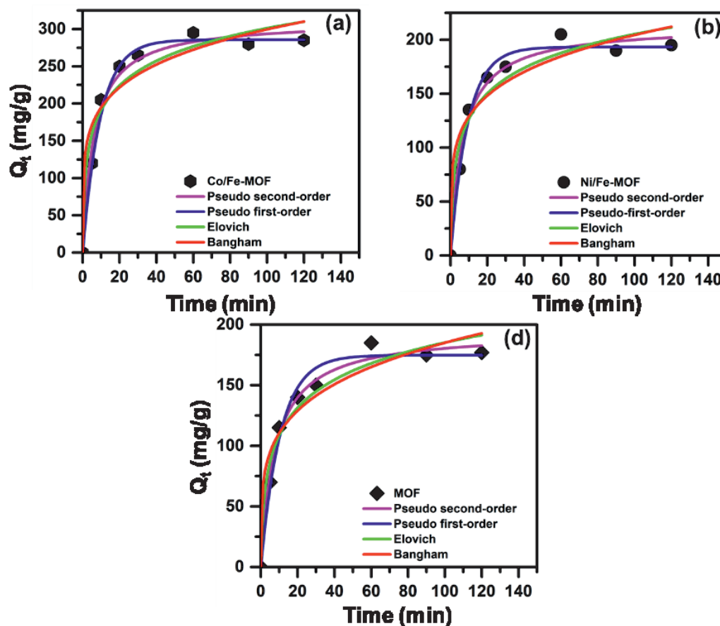
Fig. 7. The adsorption kinetic model of the materials a) Co/Fe-MOF, b) Ni/Fe-MOF, c) Fe-MOF.
