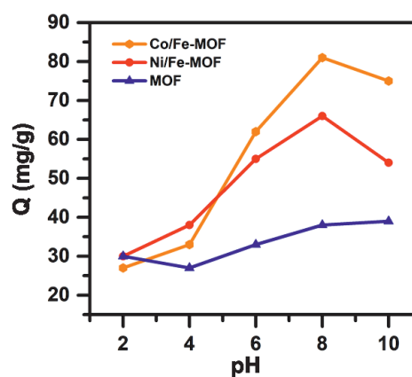
Fig. 2. Effect of pH value on the adsorption capacity of M/Fe-MOF materials (M=Co, Ni).
