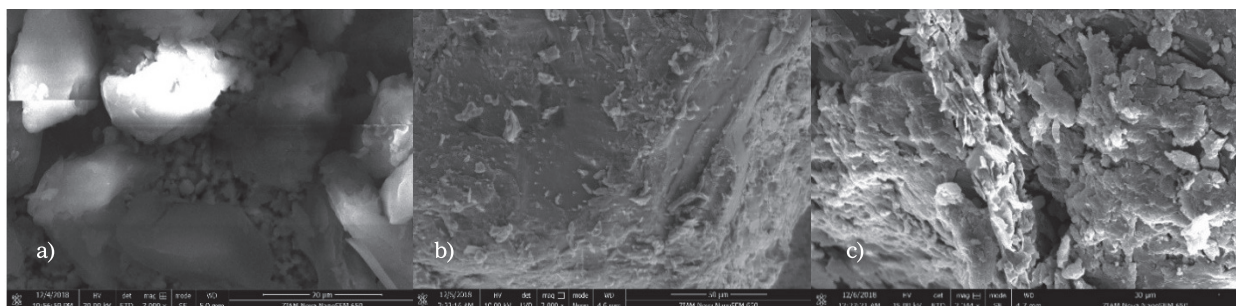
Fig. 3. The SEM micrographs of a) starch, b) poly acrylic acid and c) S-SAP.
