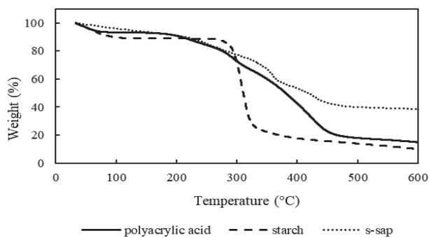
Fig. 2. The TGA curves of pure poly acrylic acid, starch and S-SAP.
