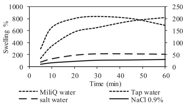
Fig. 4. The absorption capacity of SAP in water solutions with different salinities.
