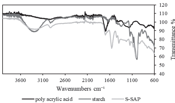
Fig. 1. The FTIR spectra of pure poly acrylic acid, starch and S-SAP.
