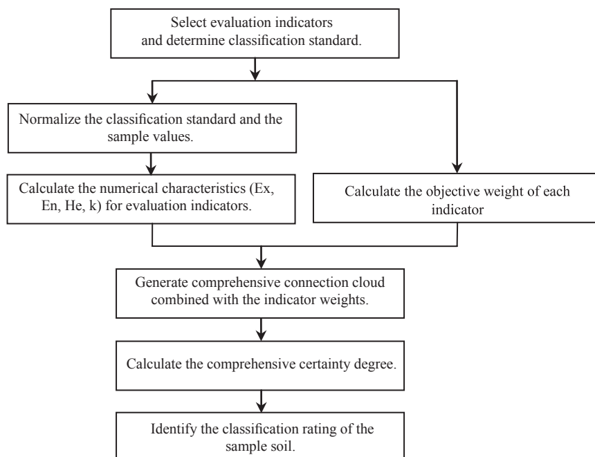
Fig. 2. Flow chart of soil heavy metal pollution evaluation based on comprehensive connection cloud model.
