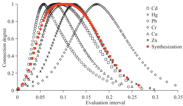
Fig.3. Clouds of each indicator and comprehensive cloud in Grade 2.
