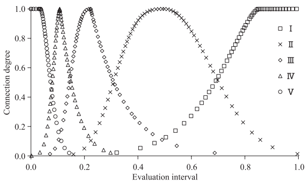
Fig.4. Comprehensive connection clouds of each grade.
