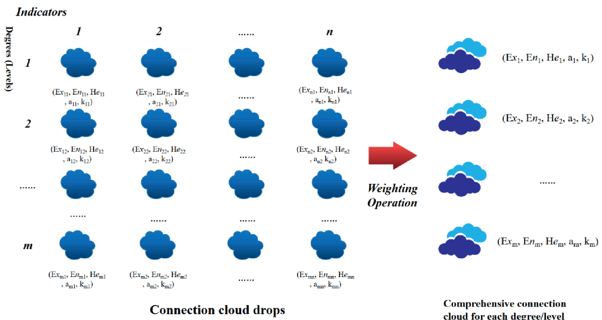
Fig. 1. Conceptual description of the comprehensive connection cloud model.
