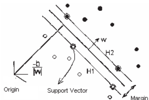
Fig. 1. Linear separation of hyperplanes for the separable case.
