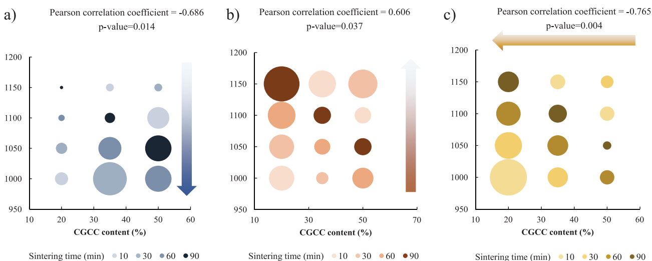
Fig. 3. The leaching toxicity of ceramsite as Cr a), As b), and Hg c). The diameter of the air bubble is positively correlated with the concentrations of trace elements (Cr, As, and Hg), and the various shades represent different sintering times.
