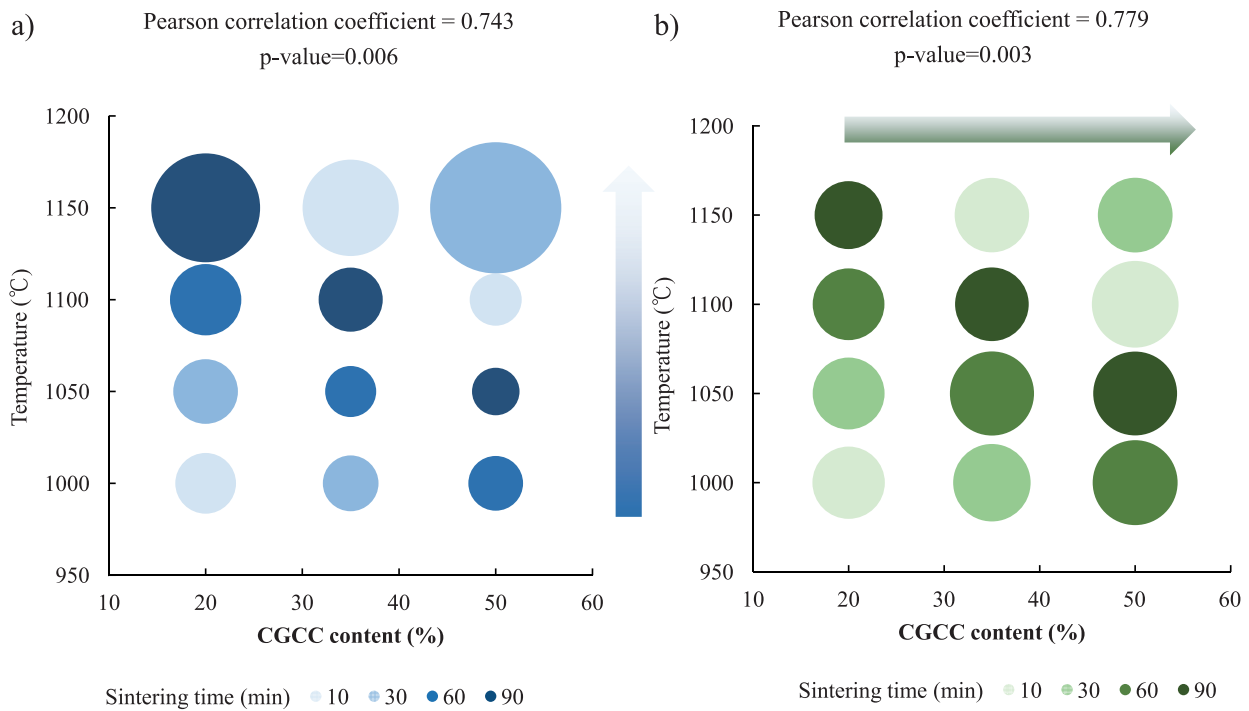
Fig. 2. Ceramsite compressive strength a) and water absorption b). The diameter of the air bubble is positively correlated with compressive strength or water absorption, and the various shades represent different sintering times.
