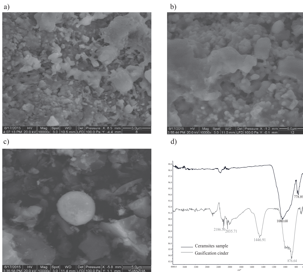
Fig. 1. SEM (10,000× magnification) of original CGCC c) and two ceramsites (a) for 35%/1150°C/10min and b) for 50%/1150°C/30min). FTIR spectrum of CGCC and ceramsite d).
