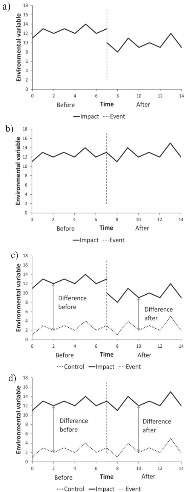
Fig. 2. Simplified data profiles for: a) BA analysis assuming impact, b) BA analysis assuming no impact, c) BACI analysis assuming impact, d) BACI analysis assuming no impact [23-24].
