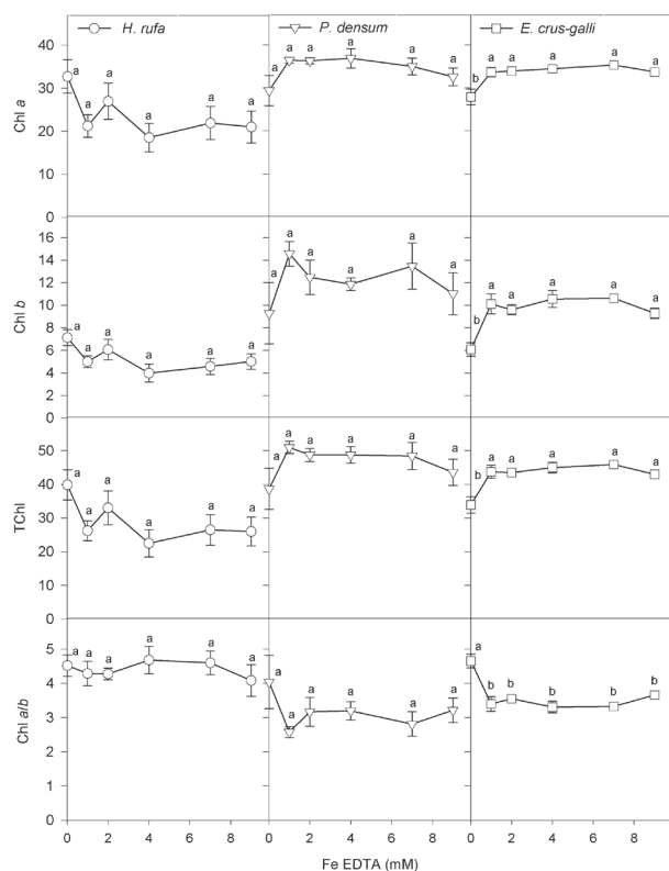
Fig. 5. Index of chlorophyll a (Chl a ), chlorophyll b (Chl b ), total chlorophyll (TChl), and ratio of chlorophyll a/b (Chl a/b ) for the grass species Hyparrhenia rufa (circle), Paspalum densum (inverted triangle), and Echinochloa crus-galli (square) briefly exposed to different concentrations of Fe-EDTA in a nutrient solution. The bars represent the mean \pm standard error of five repetitions, and means followed by the same letters for a given species do not differ by Tukey's test at the 5% significance level.
