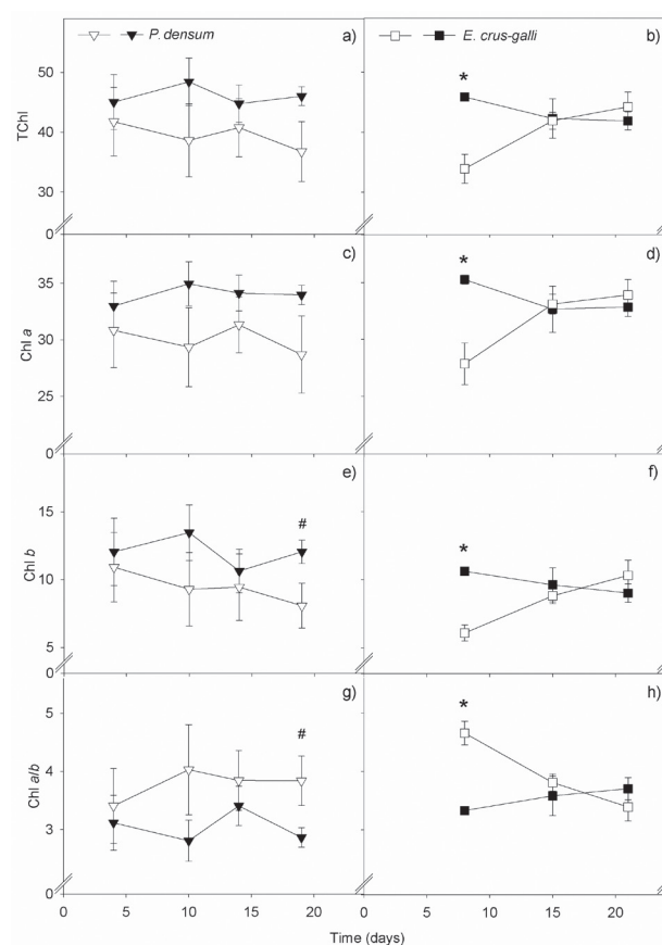
Fig. 6. Long-term changes in total chlorophyll, TChl [a) and b)], chlorophyll a , Chl a [c) and d)], chlorophyll b , Chl b [e) and f)], and the ratio of chlorophyll a/b , Chl a/b [g) and h)] for the grass species Paspalum densum (inverted triangle) and Echinochloa crus-galli (square) under control conditions (0.009 mM of Fe-EDTA; open symbol), and 7 mM of Fe-EDTA (closed symbol) in nutrient solution after 19 and 21 days of exposure, respectively. The bars indicate the mean \pm standard error of five repetitions. The symbols # and * indicate significant differences (Tukey's test, 5% probability) for P. densum and E. crus-galli , respectively.
