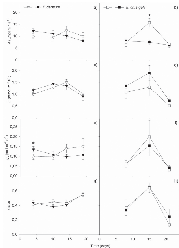
Fig. 4. Long-term changes in net photosynthetic rate, A [a and b)], transpiration, E [c) and d)], stomatal conductance, g_s [e) and f)], and the ratio between internal and external concentration of \text{CO}_2 , \text{Ci}/\text{Ca} [g) and h)] in the grass species Paspalum densum (inverted triangle), and Echinochloa crus-galli (square). Measurements were taken after 19 and 21 days, respectively, in nutrient solution under control conditions (0.009 mM of Fe-EDTA; open symbols), and 7 mM of Fe-EDTA (closed symbols). The bars indicate the mean \pm standard error of five repetitions. The symbols # and * indicate significant differences (Tukey's test, 5% probability) for P. densum and E. crus-galli , respectively.
