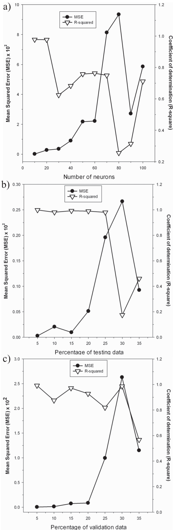
Fig. 2. Values of MSE and R-squared due to the variation of a) number of neurons, b) percentage of testing data, and c) percentage of validation data.
