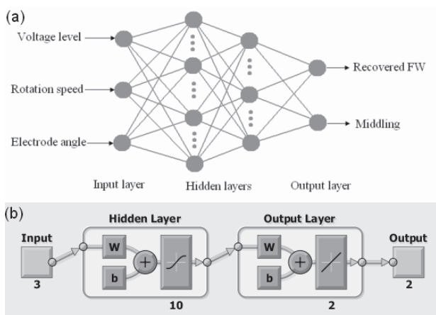
Fig. 1. Topology of the backpropagation ANN in a) schematic view and b) Matlab environment.
