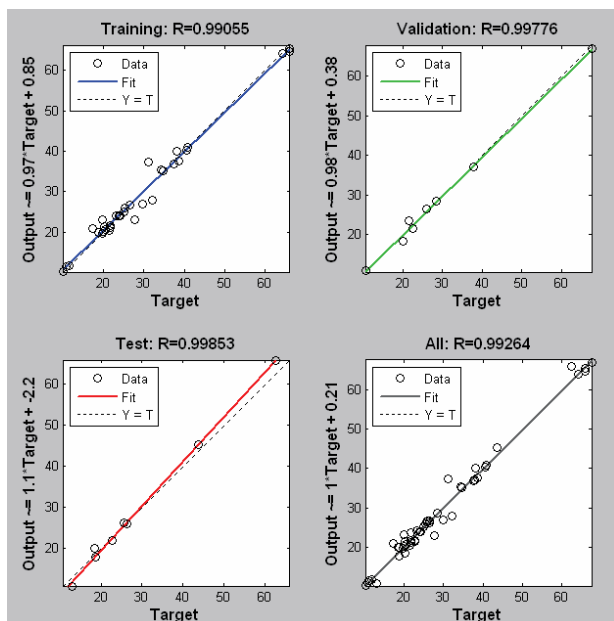
Fig. 4. Parity plots of training, testing, and validation stages.
