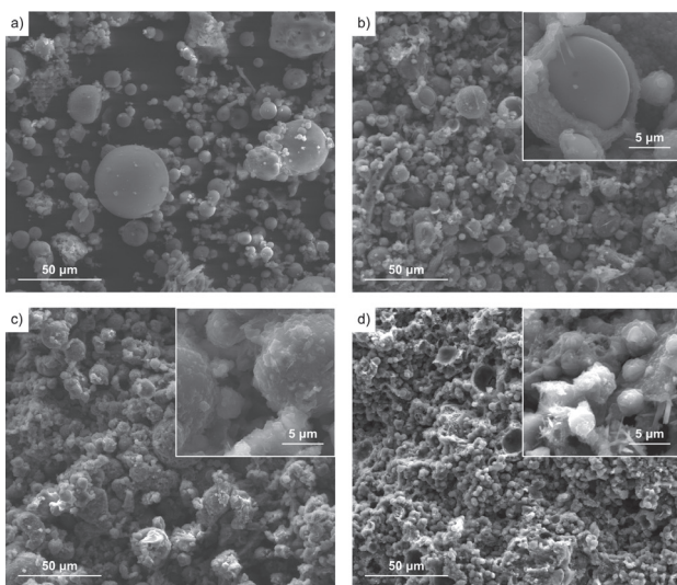
Fig. 6. SEM observations of the samples: a) fly ash, b) A_2:1, c) A_1:1, and d) B_1:1.
