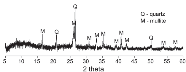
Fig. 1. XRD pattern of initial coal fly ash.
