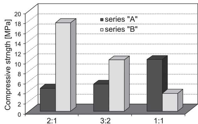
Fig. 7. Compressive strength of fly ash geopolymers.
