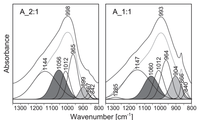
Fig. 5. Decomposition of the FT-IR spectra of the samples: a) A_2:1 and b) A_1:1.
