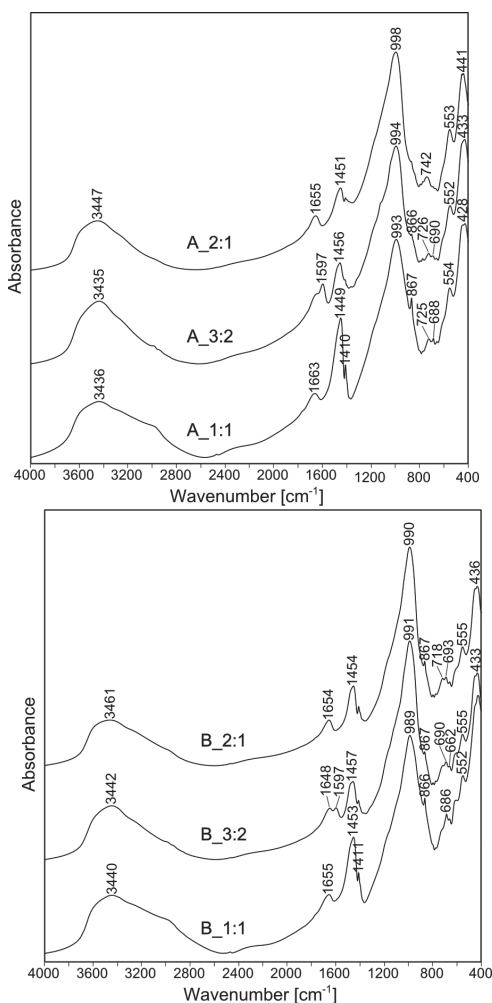
Fig. 4. FT-IR spectra of fly ash after the geopolymerization process.
