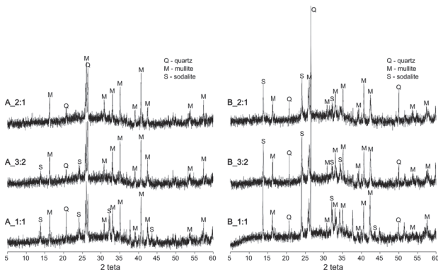
Fig. 3. XRD pattern of fly ash after the geopolymerization process.
