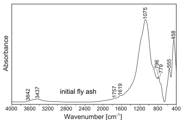
Fig. 2. MIR spectrum of initial coal fly ash.
