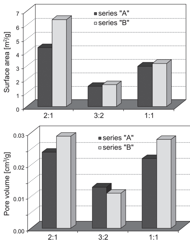
Fig. 8. BET surface area [m 2 /g] and BJH pore volume of pores between 1.7-300.0 nm (cm 3 /g) of fly ash geopolymers.
