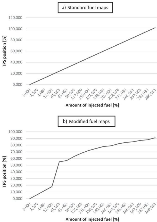
Fig. 3. Presentation of the standard and modified fuel maps.
