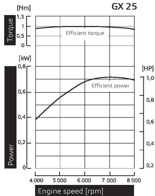
Fig. 1. Performance characteristics of the experimental engine.
