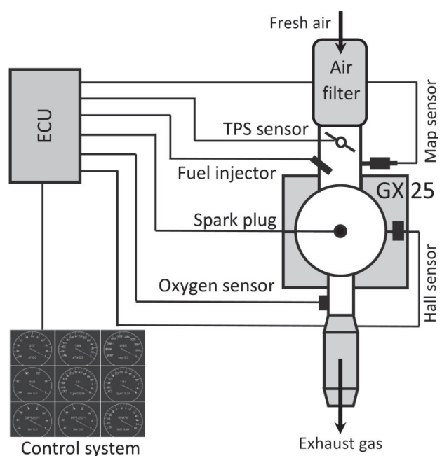
Fig. 2. Applying the EFI system for the experimental engine.
