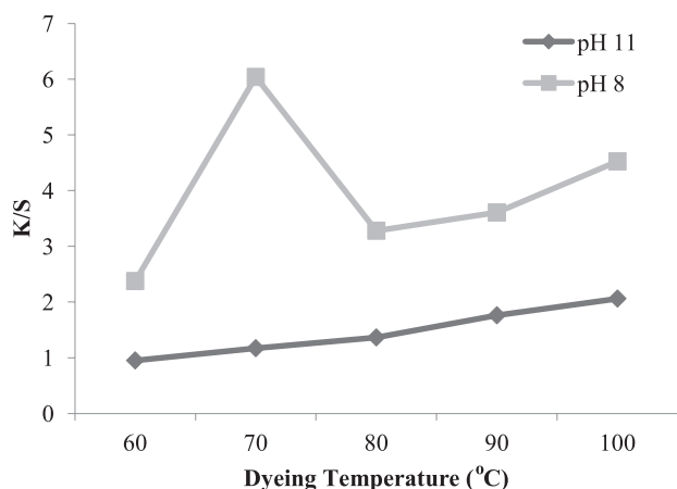
Fig. 2. Impact of dyeing temperature on k/s value of fabric dyed under optimal radiation conditions.
