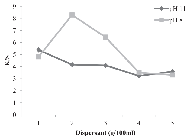
Fig. 4. Effect of dispersant on k/s of polyester fabric dyed under optimal radiation conditions.
