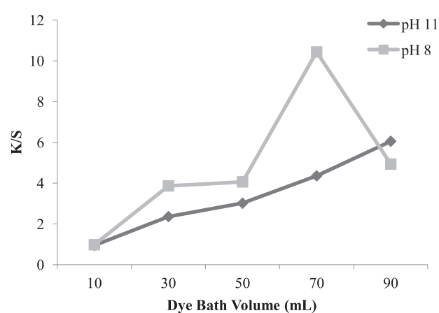
Fig. 5. Effect of dye bath volume on k/s value of polyester fabric dyed under optimal radiation conditions.
