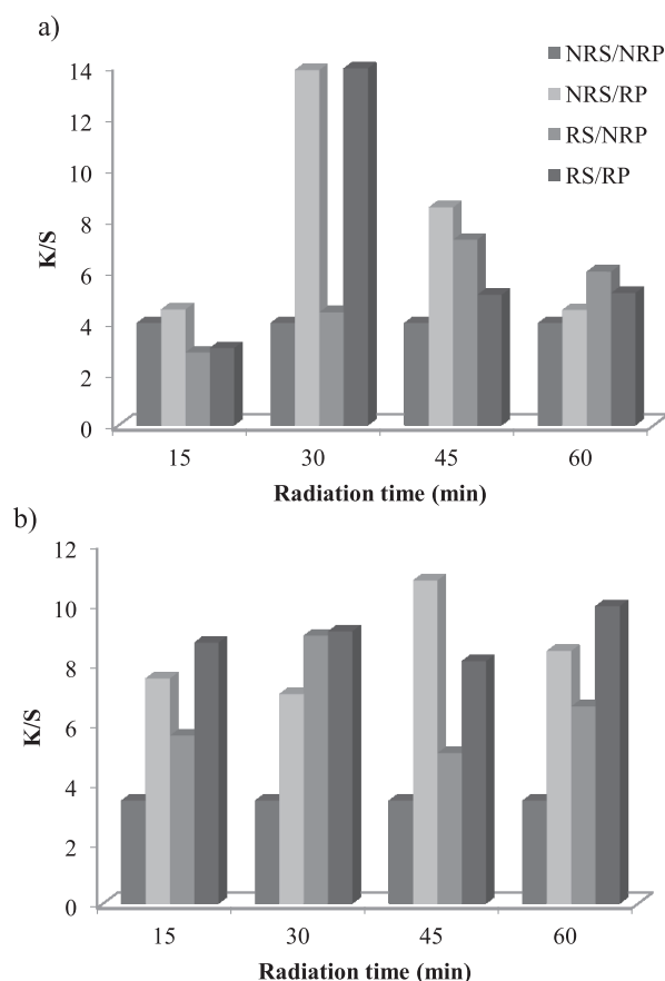
Fig. 1. Effect of ultraviolet treatment on dyeing of polyester fabrics at pH 8 a) and pH 11 b) using disperse yellow 211.
