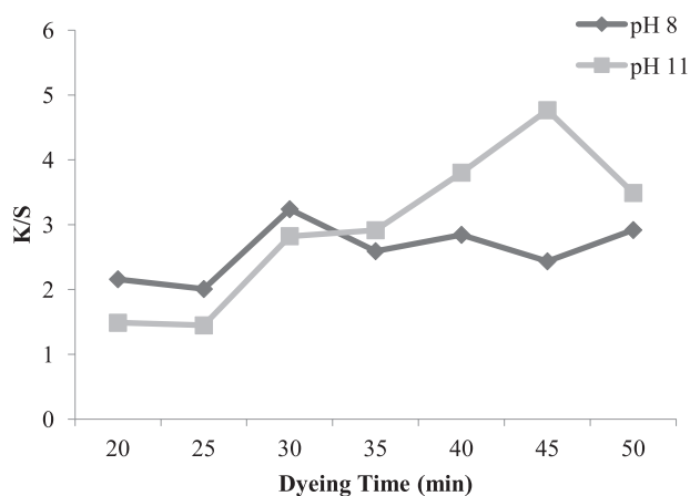
Fig. 3. Role of dyeing time on k/s value of polyester fabric dyed using optimal radiation conditions.
