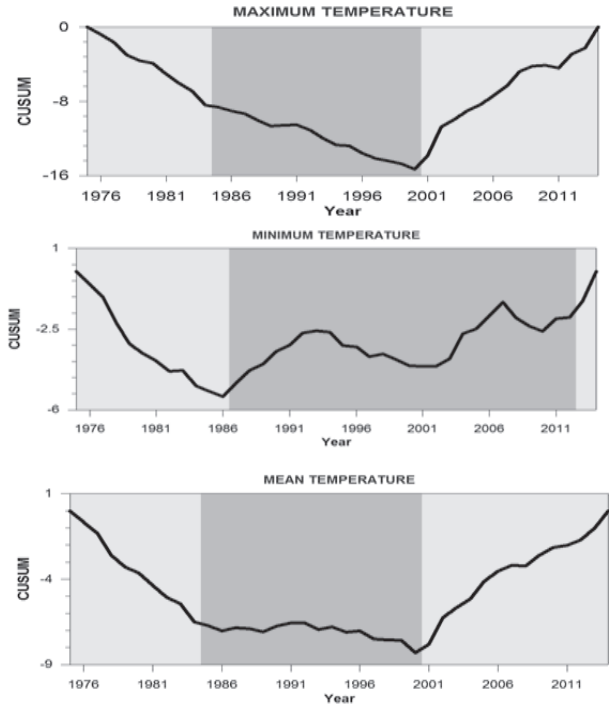
Fig. 5. CUSUM chart for annual temperature.
