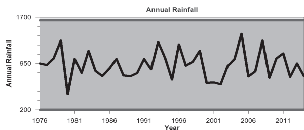
Fig. 6. Estimated change point years for annual rainfall.
