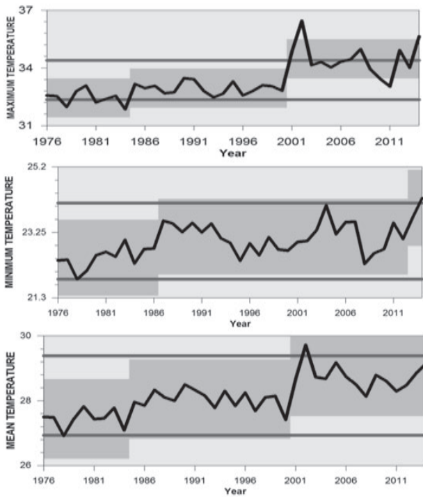
Fig. 3. Identifying change points for annual temperature.
