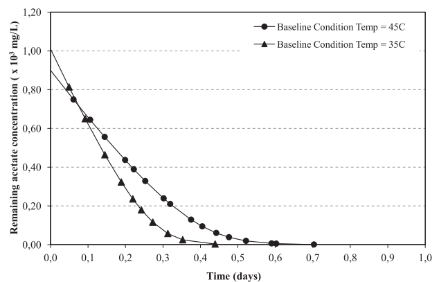
Fig. 1. Progress curve of acetate degradation at 35°C and 45°C. Different temperatures: r_{\max} (t-test, \alpha = 0.05 , p = 0.012 for \mu_{45} = \mu_{35} ), K_s (t-test, \alpha = 0.05 , p = 0.397 for \mu_{45} = \mu_{35} ).
