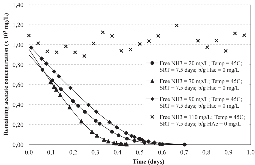
Fig. 3. Progress curve of acetate degradation at different free NH 3 concentrations of 20, 70, 90, and 110 mg/L (Temp = temperature; b/g = background).
