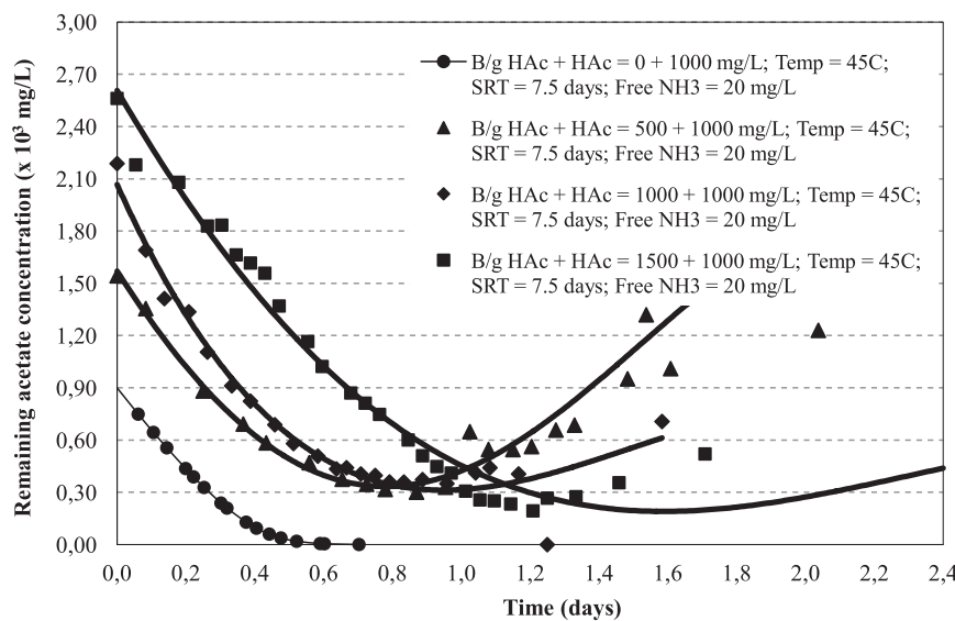
Fig. 4. Progress curve and trendline of acetate degradation at different background acetate concentrations of 0, 500, 1000, and 1500 mg/L (with the addition of synthetic acetate).
