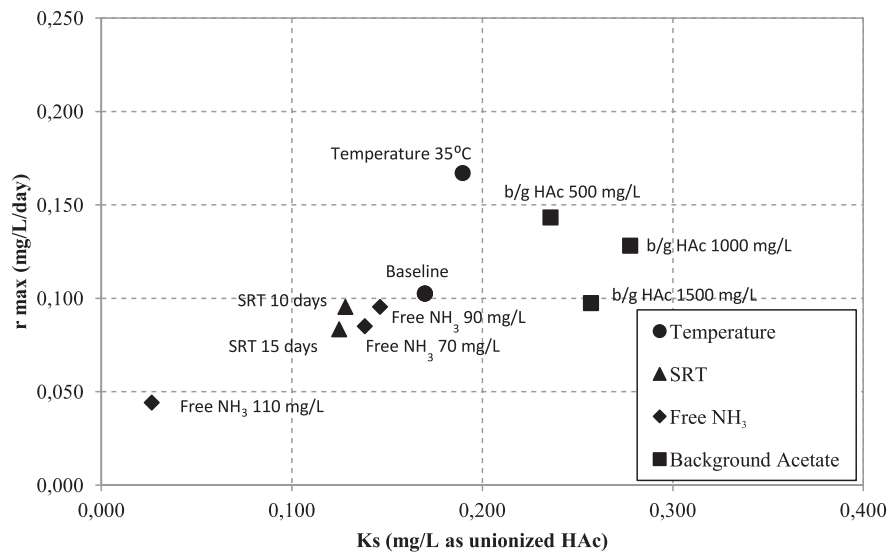
Fig. 5. K_s and r_{max} at different temperatures, SRTs, free NH_3 , and background acetates.
