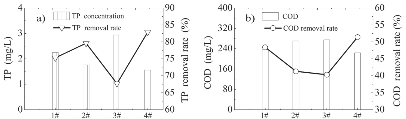
Fig. 2. TP and COD removal efficiencies under single coagulants: 1) Ferric chloride, FeCl_3 ; 2) Aluminum chloride, AlCl_3 ; 3) Ferric sulfate, Fe_2(SO_4)_3 ; and 4) compounded coagulants composed of AlCl_3 , FeCl_3 , and Fe_2(SO_4)_3 .
