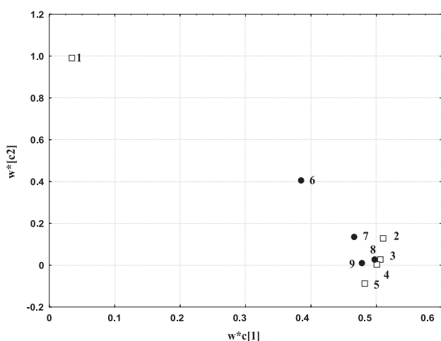
Fig. 2. The weights of the first two components of the PLS2 model ( w^*c1 , w^*c2 ). The meaning of labels: 1 – bp(BSR), 2 – bp, 3 – proteins, 4 – spirometry, 5 – Cr status, 6 – CEA, 7 – CYFRA 21-1, 8 – NSE, 9 – SCC-Ag.
