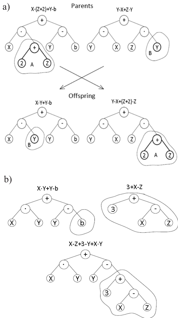
Fig. 1. Schematic activity of genetic operators for crossover a) and mutation b).
