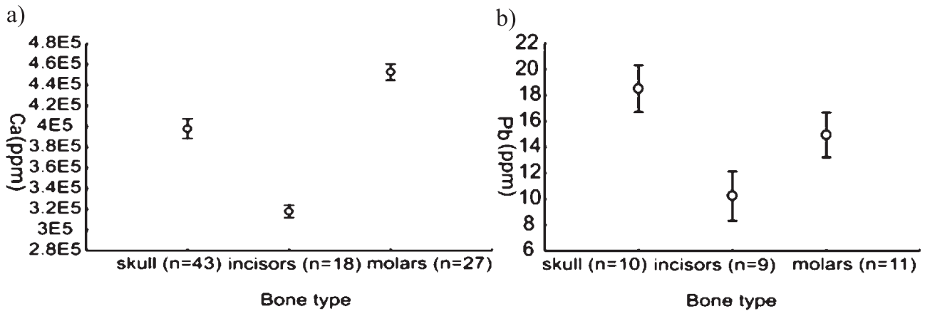
Fig. 1. A: Marmot molars contained more calcium than incisors or skull bones (one-way ANOVA, F(2, 85) = 96.22, p = 0.00001 ). All groups differ at p < 0.05 (Tukey HSD test). B: Pb levels are higher in skull bones of marmots than in their molars and incisors (one-way ANOVA, F(2, 27) = 4.98, p = 0.01 ). All groups differ at p < 0.05 (Tukey HSD test).
