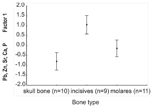
Fig. 2. Means with 0.95 confidence limits of the factor 1 scores (one-way ANOVA, F(2, 27) = 17.8 , p = 0.00001 ). Pb, Zn, Sr, Ca and P are accumulated more intensively in the skull bones than in the molars (lower numbers at y-axis mean higher levels of element concentrations, Tukey HSD test). The lowest concentration of these elements was in incisors.
