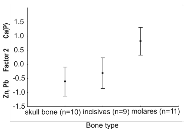
Fig. 3. Means with 0.95 confidence limits of the factor 2 scores (one-way ANOVA, F(2, 27) = 9.5 , p = 0.00075 ). The mutual concentration of lead and zinc was proportionally higher in skull bones and incisors than in molars when related to the amount of calcium (Tukey HSD test).
