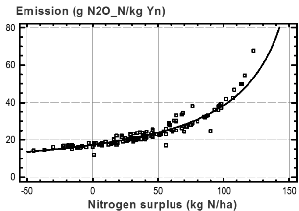
Fig. 3. Regression between yield-scaled N 2 O_N emissions (Eys) and nitrogen surplus (Ns) ( Eys = 1/(0.0577 - 0.000317 * Ns) ).
