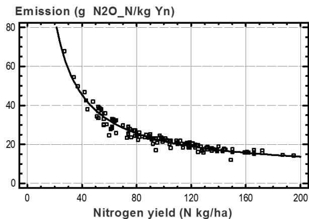
Fig. 1. Regression between yield-scaled N 2 O_N emissions (Eys) and nitrogen yield (Yn) ( Eys = 5.78 + 1587/Yn ).
