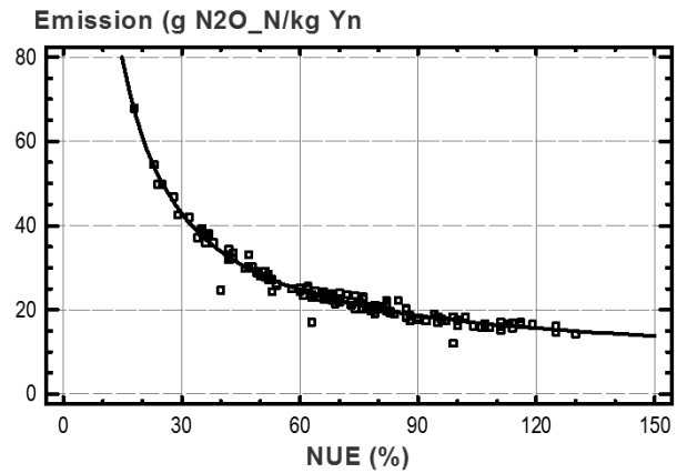
Fig. 2. Regression between yield-scaled N 2 O_N emissions (Eys) and nitrogen use efficiency (NUE) ( Eys = 6.52 + 1091/NUE ).
