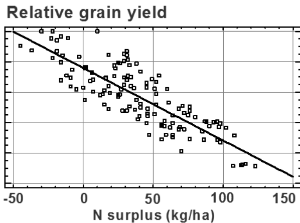
Fig. 4. Regression between relative grain yield (seeds) ( Y_g relative) and nitrogen surplus ( N_s , \text{kg ha}^{-1} ) ( Y_g \text{ relative} = 0.759 - 0.00477 * N_s ; r^2 = 69.5\% ).
