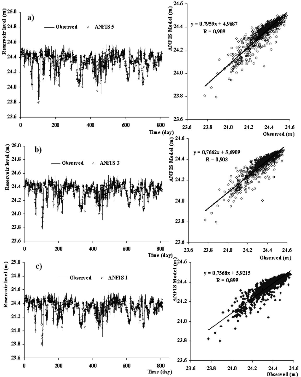
Fig. 7. Observed and predicted reservoir levels for Millers Dam in the test period: a) ANFIS5, b) ANFIS3, and c) ANFIS1.
