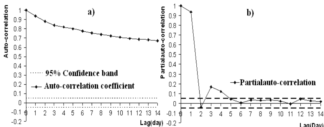
Fig. 6. a) Autocorrelation and b) partial auto-correlation functions of daily reservoir levels.
