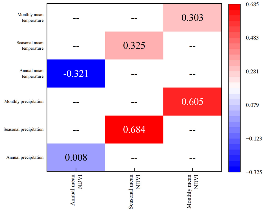
Fig. S4. Heatmap of correlations between the NDVI and climatic factors at different scales
