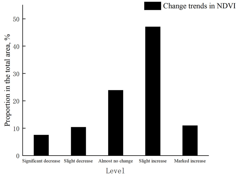
Fig. S2. The interannual change trend of NDVI in Yiliang County
