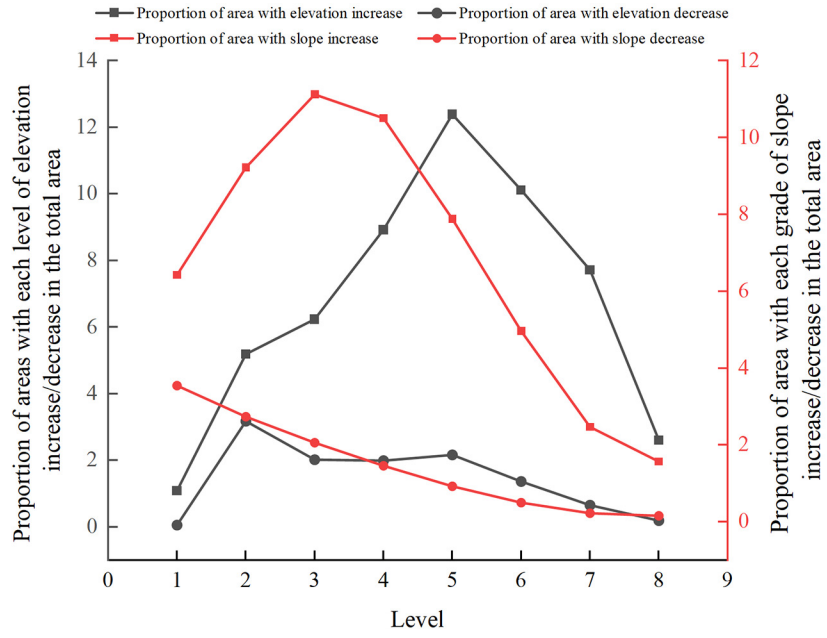
Fig. S3. Interannual NDVI change trend vs. elevation and slope
