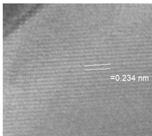
Fig S1. HRTEM image of Pd° particles on AC
