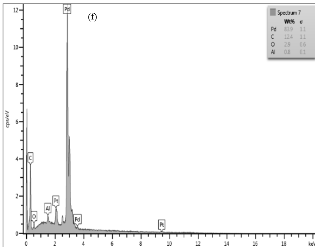
Fig. S2. EDS spectra of PdNPs reduced by (a) 2 mM BH (b) 10 mM BH, (c) 2 mM HH, (d) 10 mM HH, (e) 2 mM AA, and (f) 10 mM AA.
