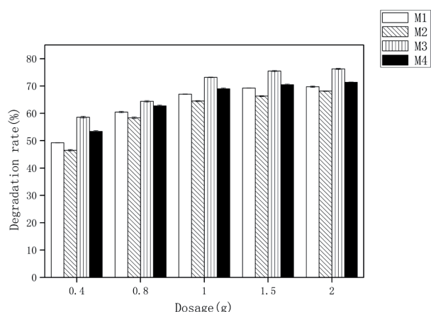
Fig. 5. Influence of dosage on immobilized strains degradation of carbofuran.
