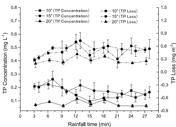
Fig. 5. Characteristics of TP concentration and loss in the surface runoff on different slope gradients.
