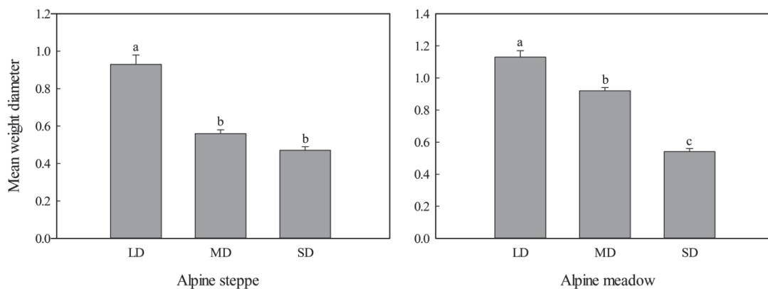
Fig. 3. Mean weight diameter of soil aggregates with different degradation levels. Different letters refer to a significant difference at the 0.05 level. MWD - mean weight diameter; LD - lightly degraded; MD - moderately degraded; SD - severely degraded.
