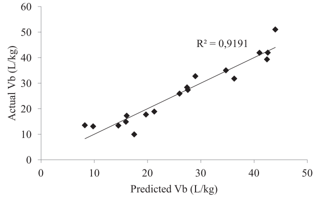
Fig. 5. Comparison of Taguchi model with experimental results for V_b .
