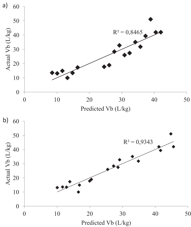
Fig. 4. Comparison of a) the linear regression model and b) quadratic regression model with experimental results for V_b .
