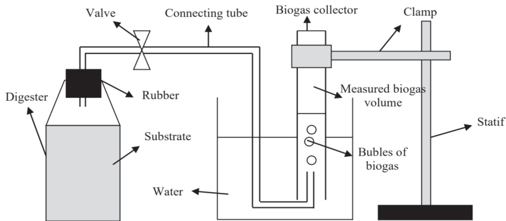
Fig. 1. The schematic diagram of the experiment.
