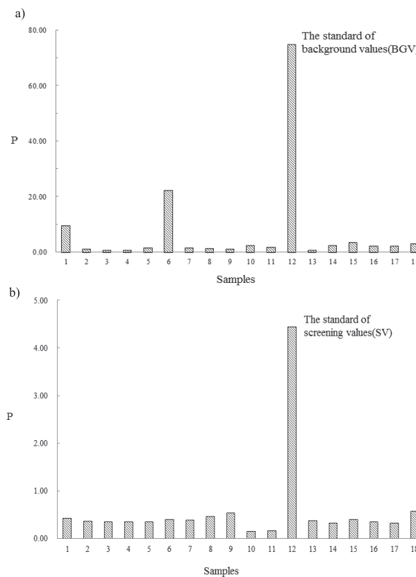
Fig. 2. Comprehensive pollution index of heavy metals in surface soils.
