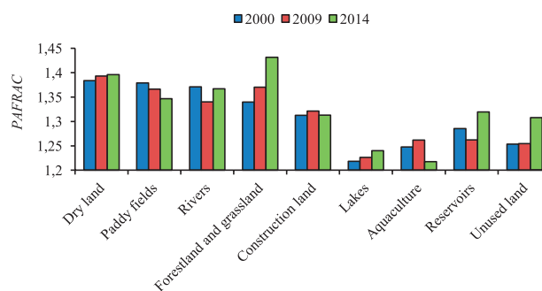
Fig. 6. PAFRAC of landscape types within the Ningde coastal zone in 2000, 2009, and 2014.
