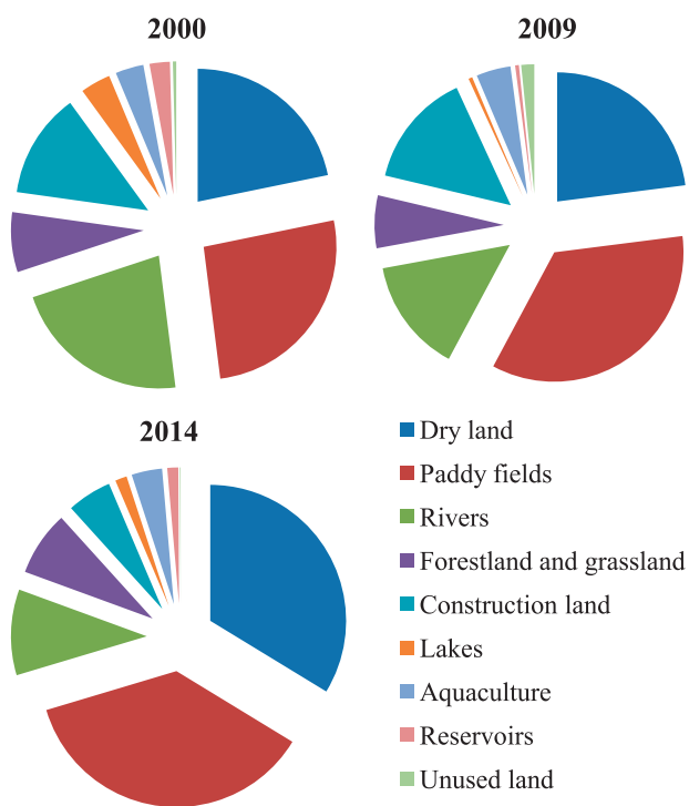
Fig. 4. Changes in the NP for the landscape types within the Ningde coastal zone.
