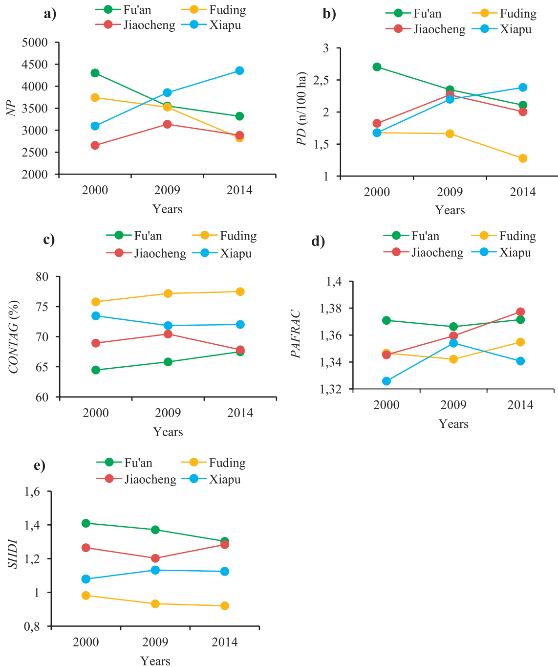
Fig. 2. Changes in the landscape indices for cities within the Ningde coastal zone.
