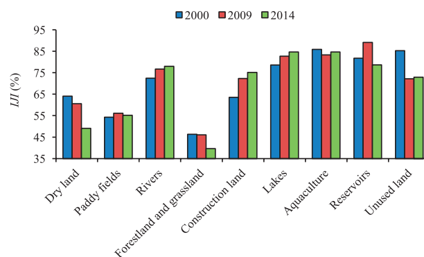
Fig. 5. IJI of landscape types within the Ningde coastal zone in 2000, 2009, and 2014.
