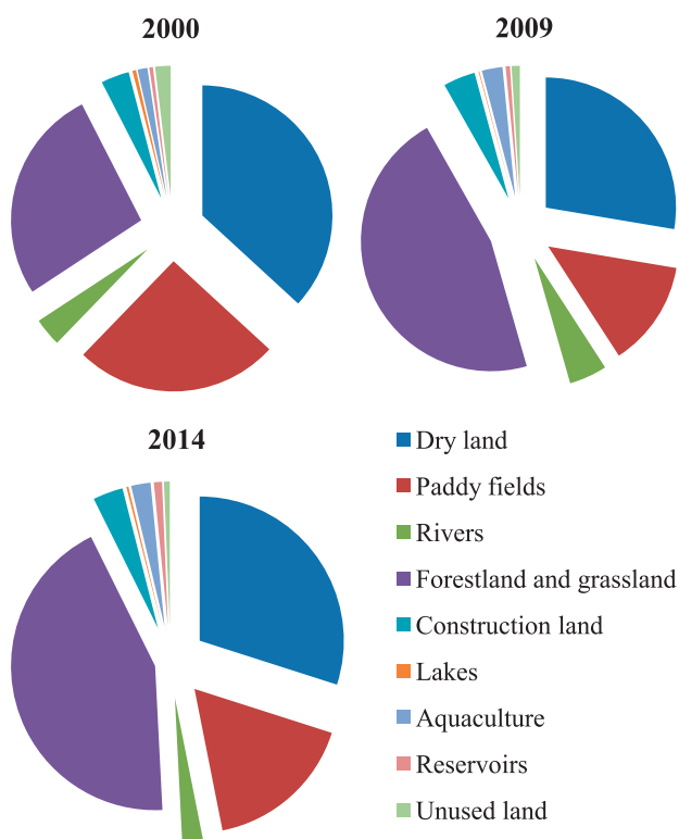
Fig. 3. Changes in the PLAND for the landscape types within the Ningde coastal zone (%).
