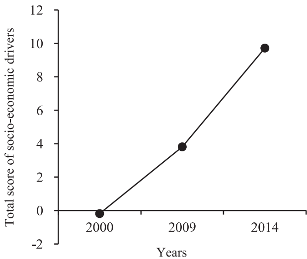
Fig. 7. Total score of socio-economic drivers influencing landscape changes in the Ningde coastal zone.
