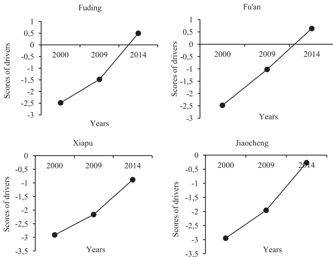
Fig. 8. Scores of drivers influencing the landscape changes on the cities within the Ningde coastal zone.
