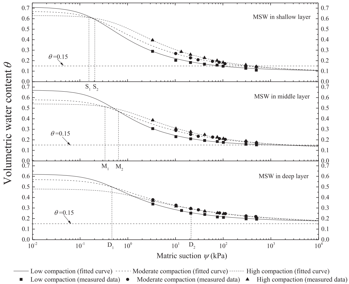
Fig. 2. SWCC of MSW under low, moderate, and high compaction.
