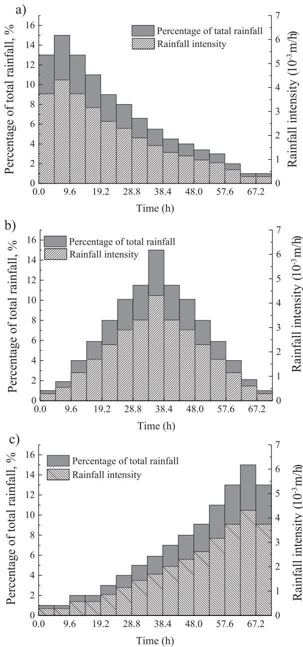
Fig. 8. Idealized rainfall patterns and rainfall intensity with total rainfall of 92.09 mm in 72 h: a) advanced rainfall pattern, b) normal rainfall pattern, and c) delayed rainfall pattern.
