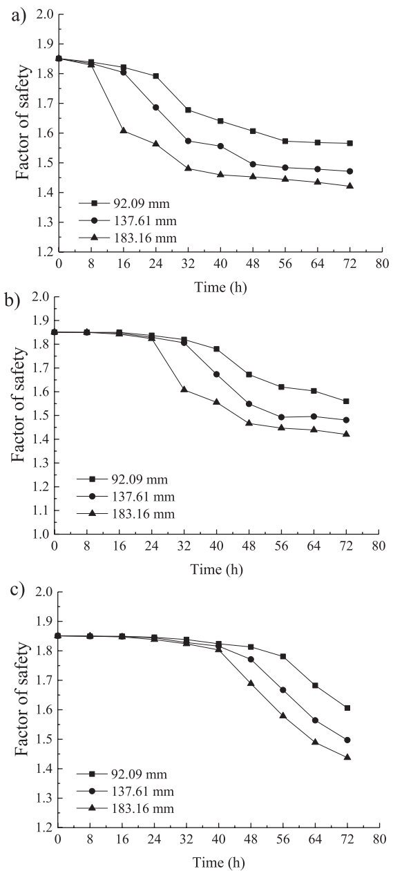
Fig. 10. Variation in the safety factor with time during different rainfall patterns at the Jianguogou landfill: a) the advanced rainfall pattern, b) the normal rainfall pattern, and c) the delayed rainfall pattern.
