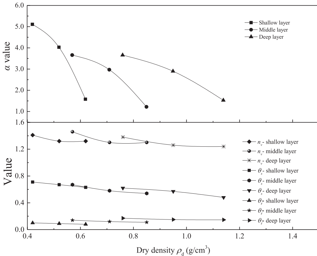
Fig. 3. Parameters of the soil water characteristic curve vs. dry density.
