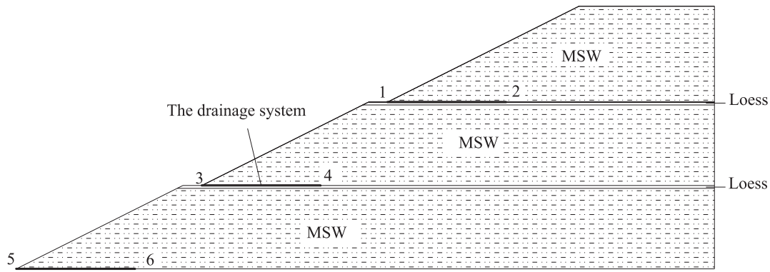
Fig. 5. Schematic diagram of the partial slope.
