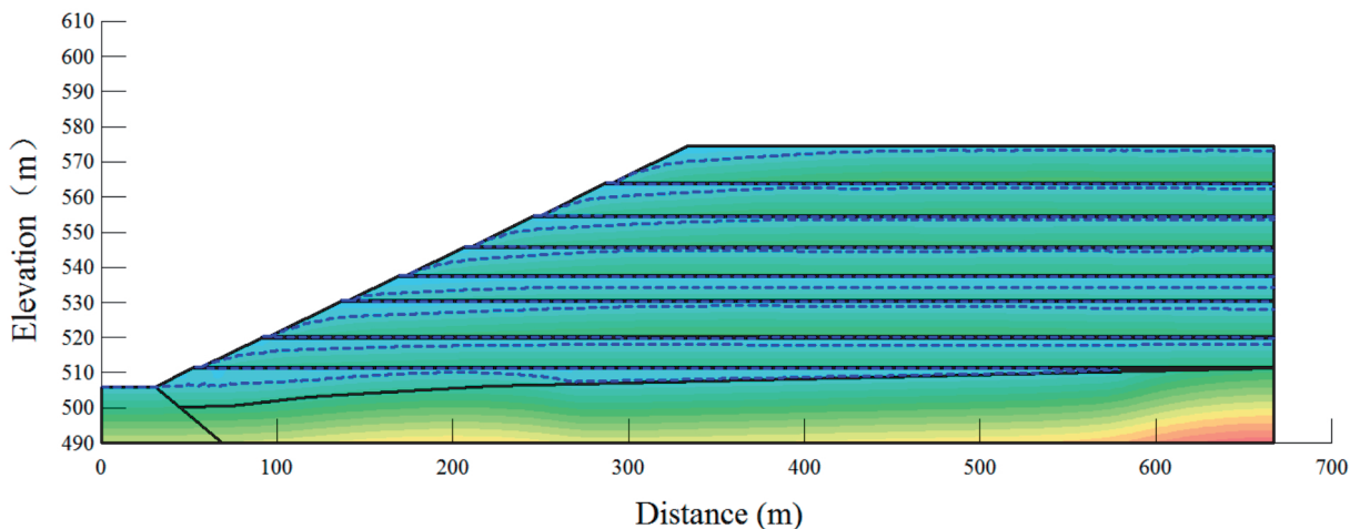
Fig. 4. The initial water level of the landfill with failed drainage, medium compaction and the slope of 1:4.0.
