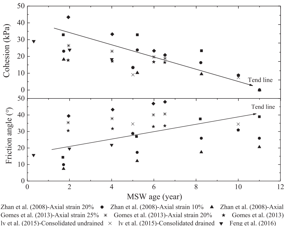
Fig. 7. Variation in the shear strength parameters of the MSW related to age [34–37].
