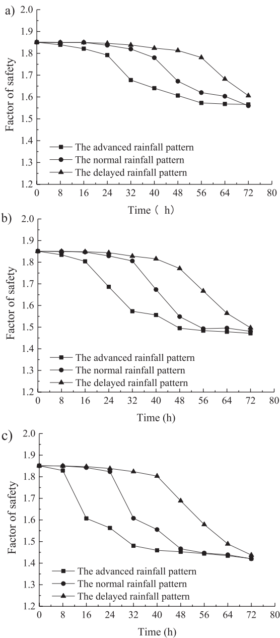
Fig. 9. Variation in the safety factor with time for the different rainfall intensities at the Jianguogou landfill: a) total rainfall of 92.09 mm within 72 hours, b) total rainfall of 137.61 mm within 72 hours, and c) total rainfall of 183.16 mm within 72 hours.
