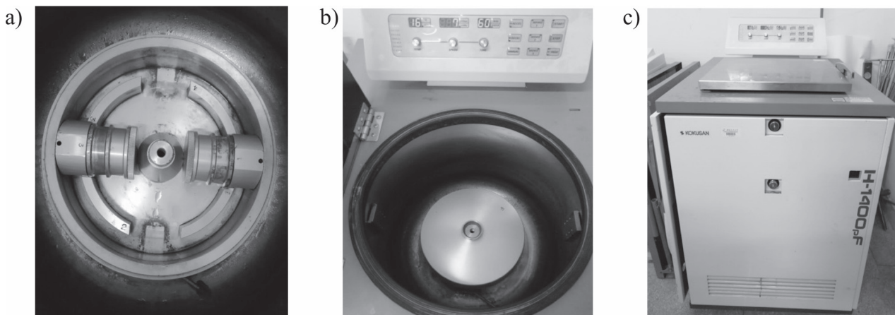
Fig. 1. The H-1400PF SWCC measurement system: a) Put centrifuge rotor into the centrifuge; b) Cover the lid; c) Close the door of the centrifuge.
