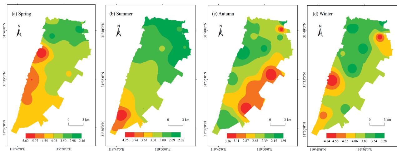
Fig. 5. Spatial distribution of the DOC concentration in spring, summer, autumn and winter in Gehu Lake.
