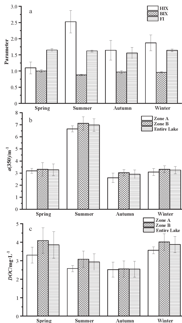
Fig. 4. The distribution of a) humification index (HIX), index of recent autochthonous biological activity (BIX), fluorescence index (FI), b) dissolved organic matter absorption coefficient at 350 nm ( a(350) ) and c) dissolved organic carbon (DOC) values in each lake.
