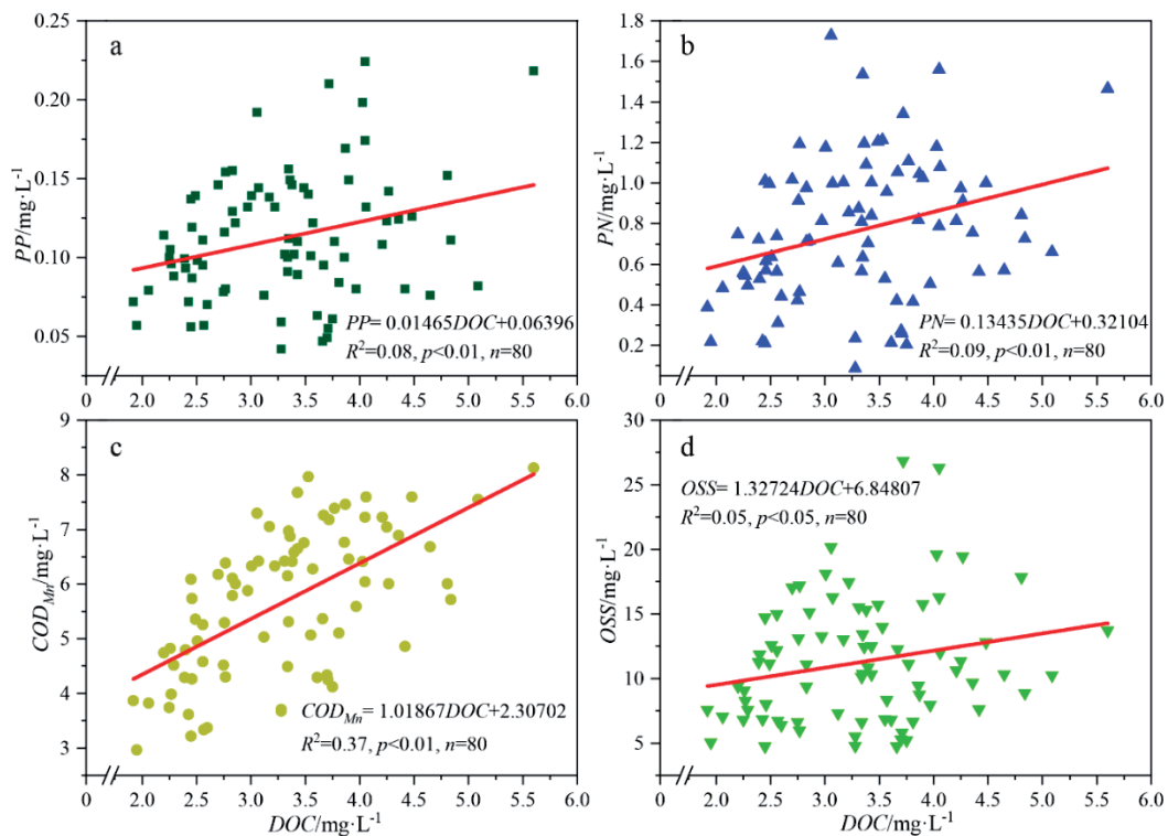
Fig. 6. Mutual correlations between a) dissolved organic carbon (DOC) and Granular phosphorus (PP), b) granular nitrogen (PN), c) permanganate index ( COD_{Mn} ), and d) organic suspended solids (OSS).
