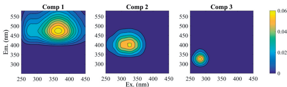
Fig. 3. Fluorescent components separated by PARAFAC.
