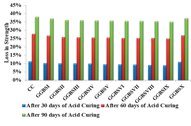
Fig. 8. Loss in Strength of specimen under Hydrochloric Acid Attack.
