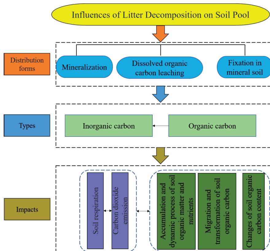
Fig. 3. Influence of litter decomposition on soil carbon pool.
