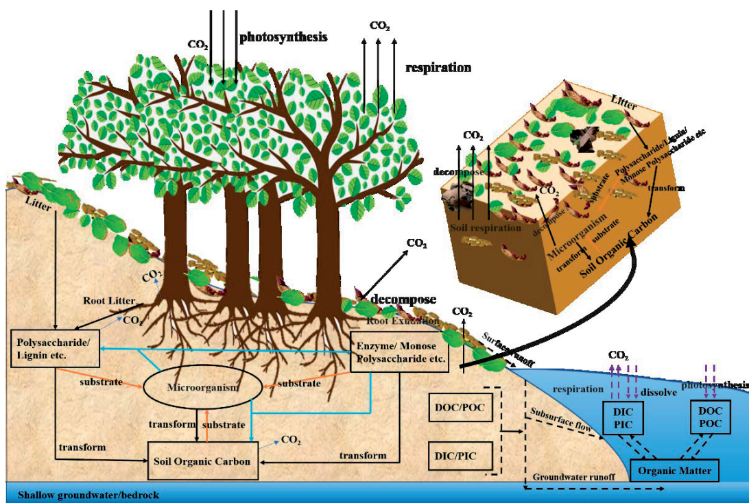
Fig. 1. Carbon cycle between litter and soil.
