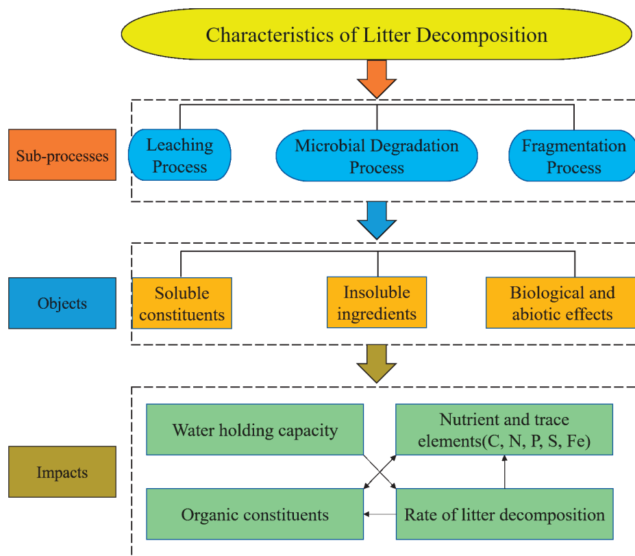
Fig. 2. Influence of litter decomposition on its characteristics.
