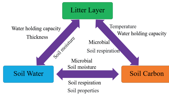
Fig. 4. Conceptual figure of interaction among litter, soil carbon and soil water.
