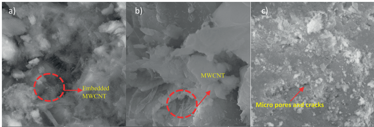
Fig. 8. SEM Images of MWCN-0.1 a) After 28 days b) after 8 weeks of chloride exposure c) after 8 weeks of sulphuric acid exposure.
