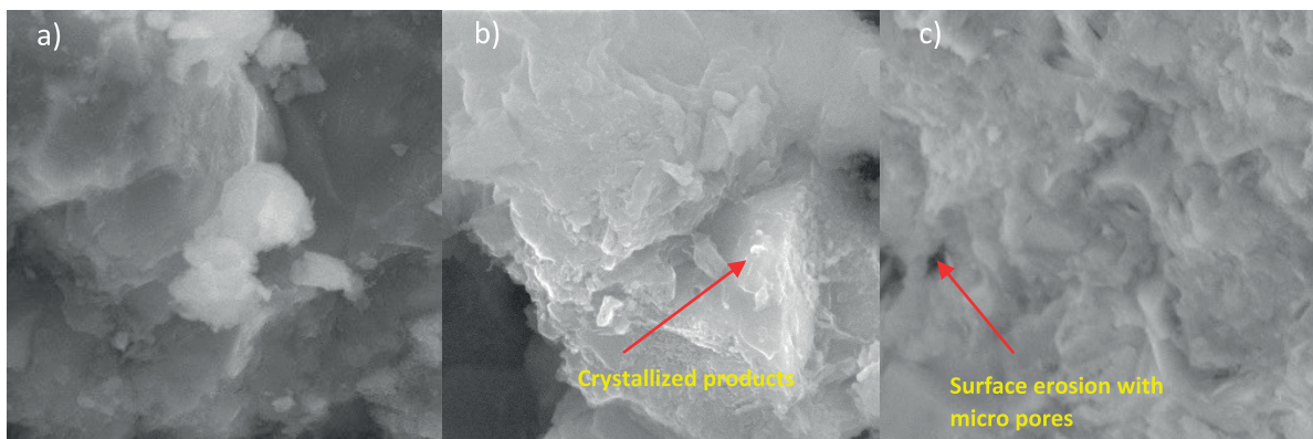
Fig. 6. SEM Images of MWCN-0 a) After 28 days b) after 8 weeks of chloride exposure c) after 8 weeks of sulphuric acid exposure.
