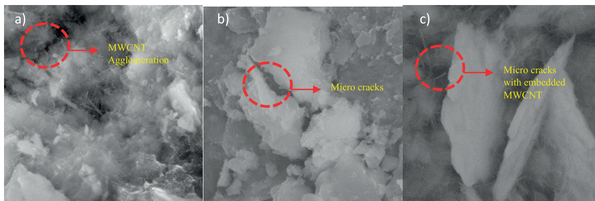
Fig. 11. SEM Images of MWCN-0.25 a) After 28 days b) after 8 weeks of chloride exposure c) after 8 weeks of sulphuric acid exposure.
