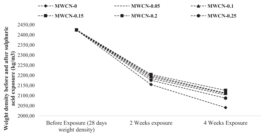
Fig. 4. Weight density before and after exposure to sulphuric acid.
