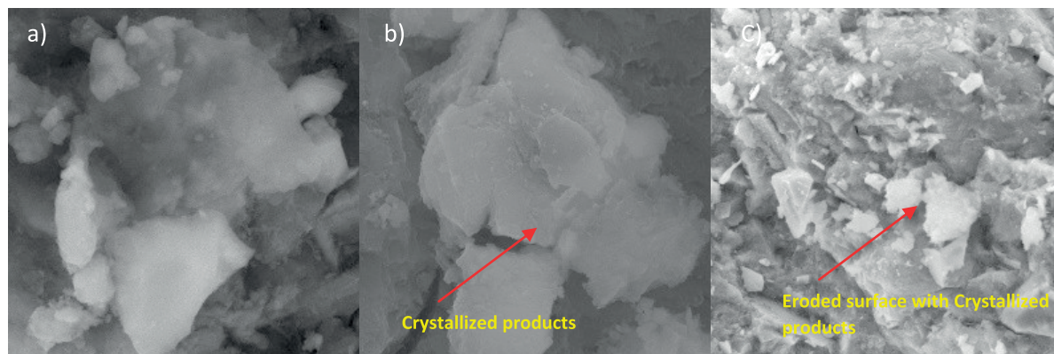
Fig. 7. SEM Images of MWCN-0.05 a) After 28 days b) after 8 weeks of chloride exposure (c) after 8 weeks of sulphuric acid exposure.
