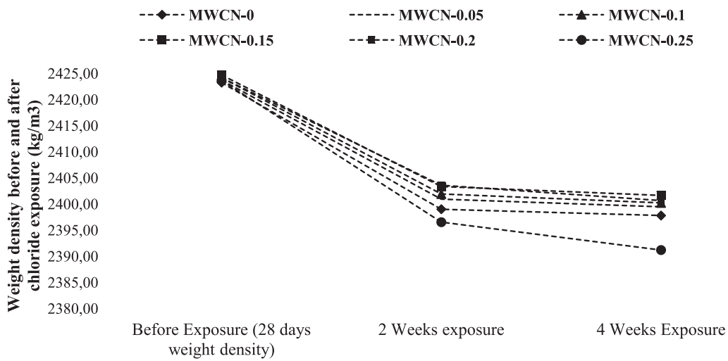
Fig. 2. Weight density before and after exposure to chloride solution.
