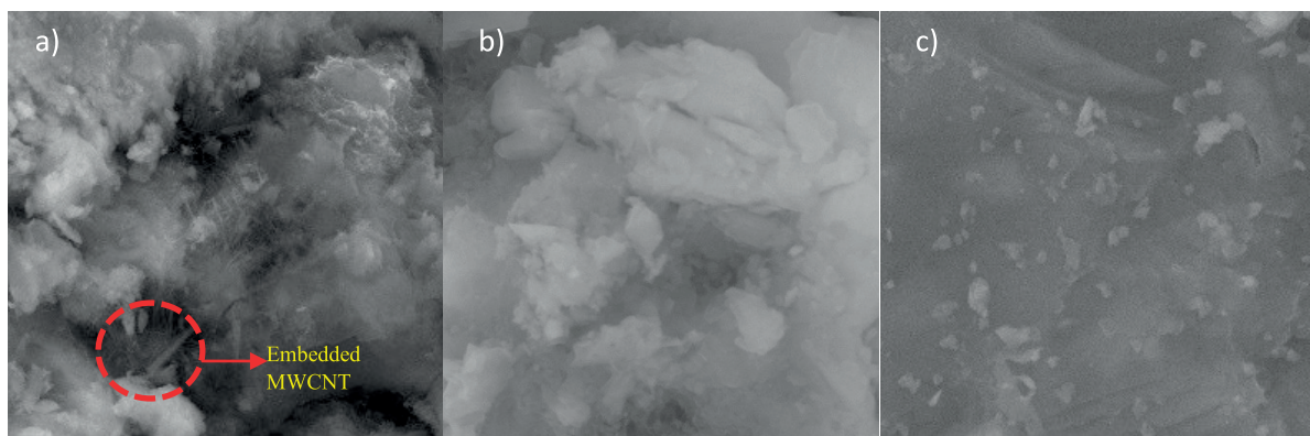
Fig. 9. SEM Images of MWCN-0.15 a) After 28 days b) after 8 weeks of chloride exposure c) after 8 weeks of sulphuric acid exposure.
