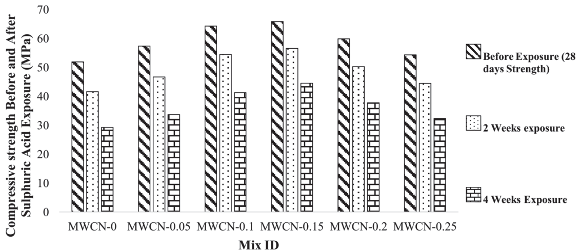
Fig. 5. Compressive strength before and after exposure to sulphuric acid.
