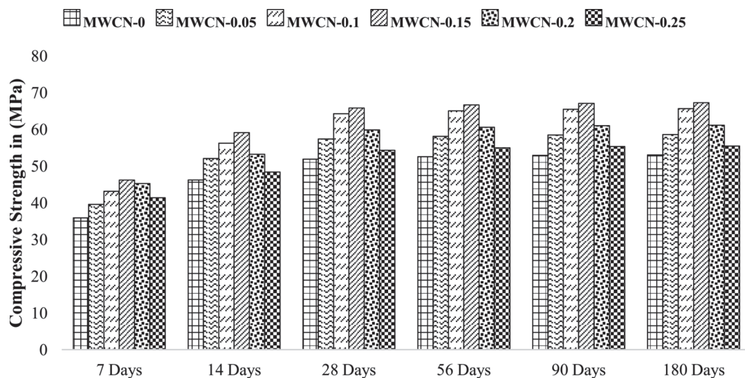
Fig. 1. Compressive strength of concrete specimens.
