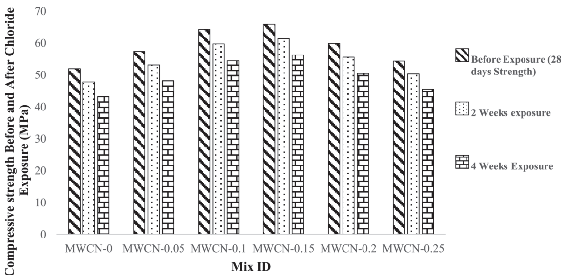
Fig. 3. Compressive strength before and after exposure to chloride solution.
