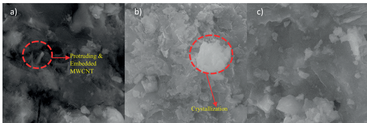
Fig. 10. SEM Images of MWCN-0.2 a) After 28 days b) after 8 weeks of chloride exposure c) after 8 weeks of sulphuric acid exposure.
