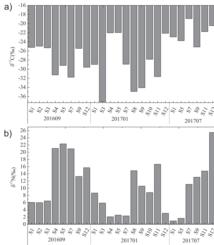
Fig. S3. Variations of ^{13}\text{C} a) and ^{15}\text{N} b) in periphyton collected from Pearl River between Guongzhou and Humen (S1-S12: sampling sites see Fig. S1).
