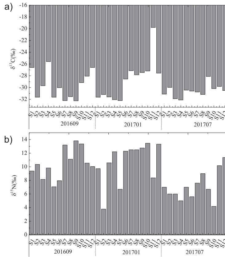
Fig. S2. Variations of ^{13}\text{C} a) and ^{15}\text{N} b) in suspended particulate organic matter (POM) collected from Pearl River between Guongzhou and Humen (S1-S12: sampling sites see Fig. S1).
