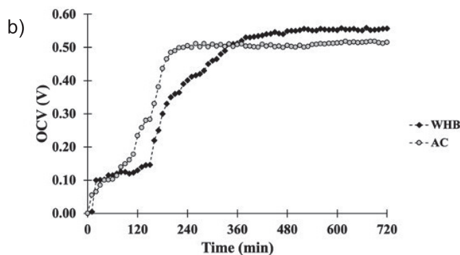
Fig. 1. The activated WHB was used in this experiment a), and the opened-circuit voltage (OCV) was gained from the CMFC with the WHB and AC electrode b).
