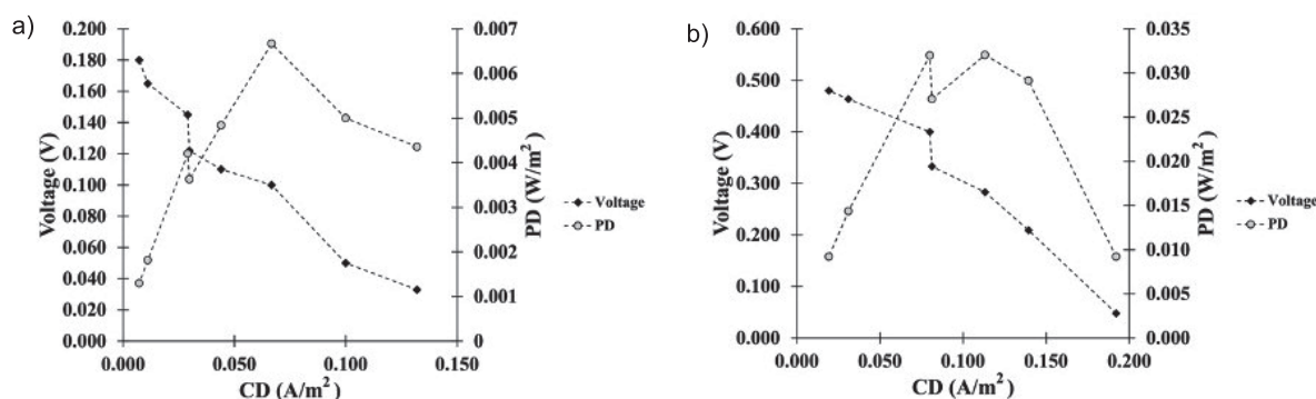
Fig. 2. The polarization curve of the CMFC with the WHB a) and AC b).
